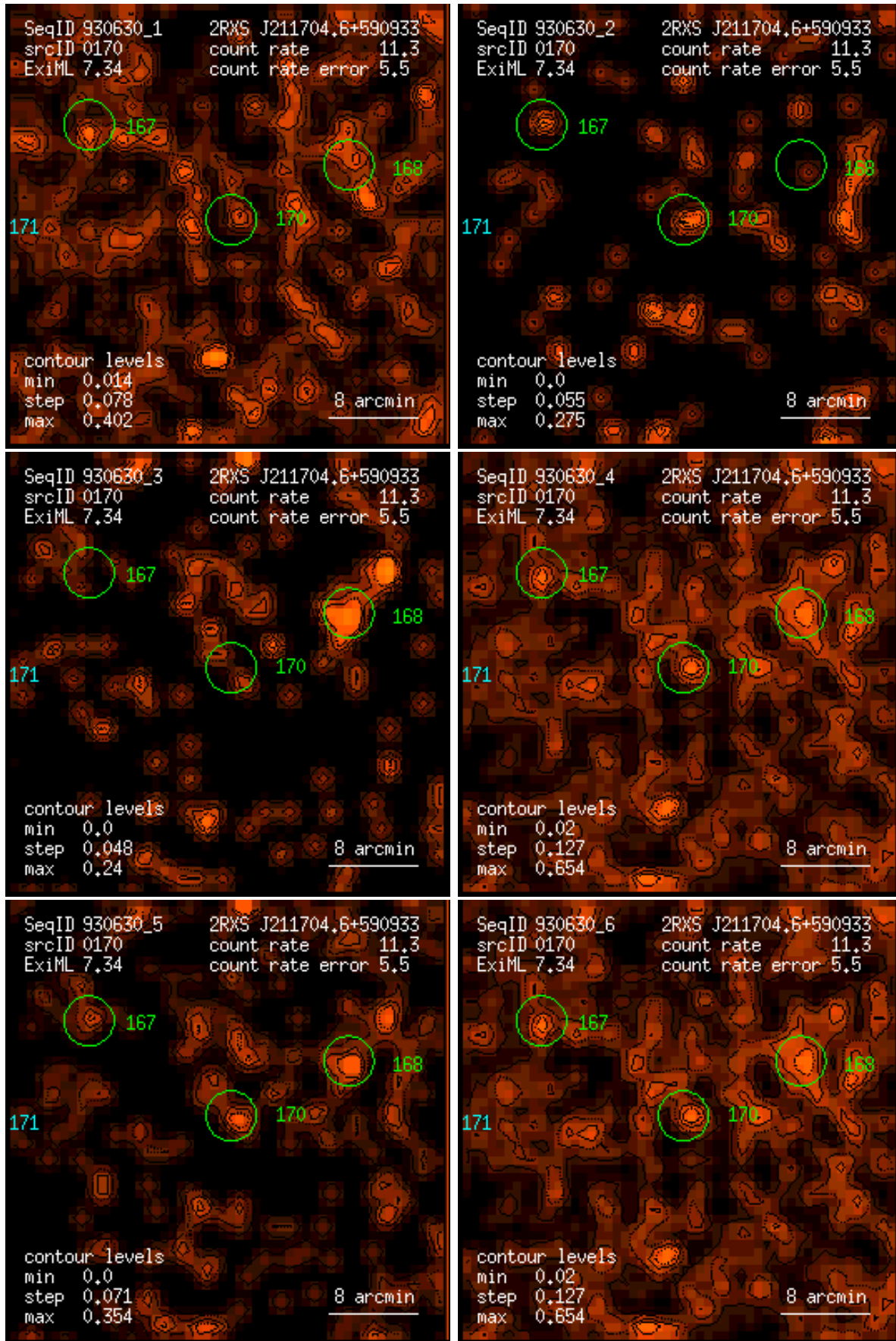
Figure 170: RASS 930630: detection 0170: band rate images, Gaussian filter: (1) PSPC channels 11 – 41, (2) 52 – 90, (3) 91 – 201, (4) 11 – 235, (5) 52 – 201, (6) 11 – 201. Broad band rates in counts/ks. Band rate contour levels in counts/ks/arcmin 2 .
