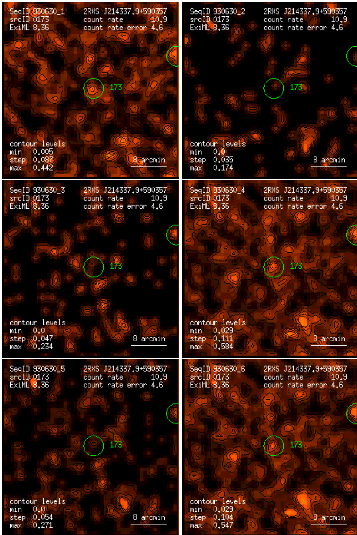
Figure 173: RASS 930630: detection 0173: band rate images, Gaussian filter: (1) PSPC channels 11 – 41, (2) 52 – 90, (3) 91 – 201, (4) 11 – 235, (5) 52 – 201, (6) 11 – 201. Broad band rates in counts/ks. Band rate contour levels in counts/ks/arcmin 2 .
