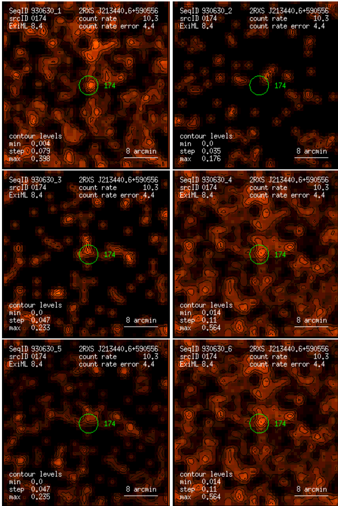
Figure 174: RASS 930630: detection 0174: band rate images, Gaussian filter: (1) PSPC channels 11 – 41, (2) 52 – 90, (3) 91 – 201, (4) 11 – 235, (5) 52 – 201, (6) 11 – 201. Broad band rates in counts/ks. Band rate contour levels in counts/ks/arcmin 2 .
