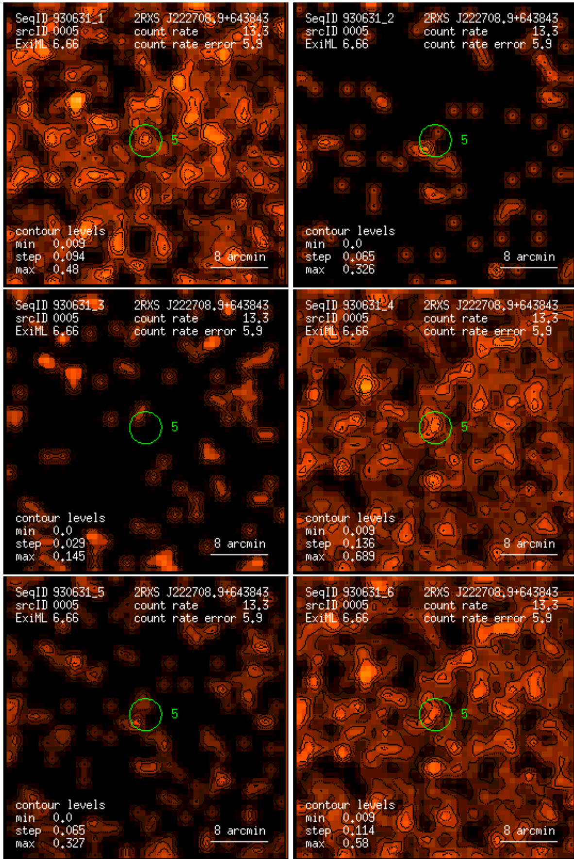
Figure 5: RASS 930631: detection 0005: band rate images, Gaussian filter: (1) PSPC channels 11 – 41, (2) 52 – 90, (3) 91 – 201, (4) 11 – 235, (5) 52 – 201, (6) 11 – 201. Broad band rates in counts/ks. Band rate contour levels in counts/ks/arcmin 2 .
