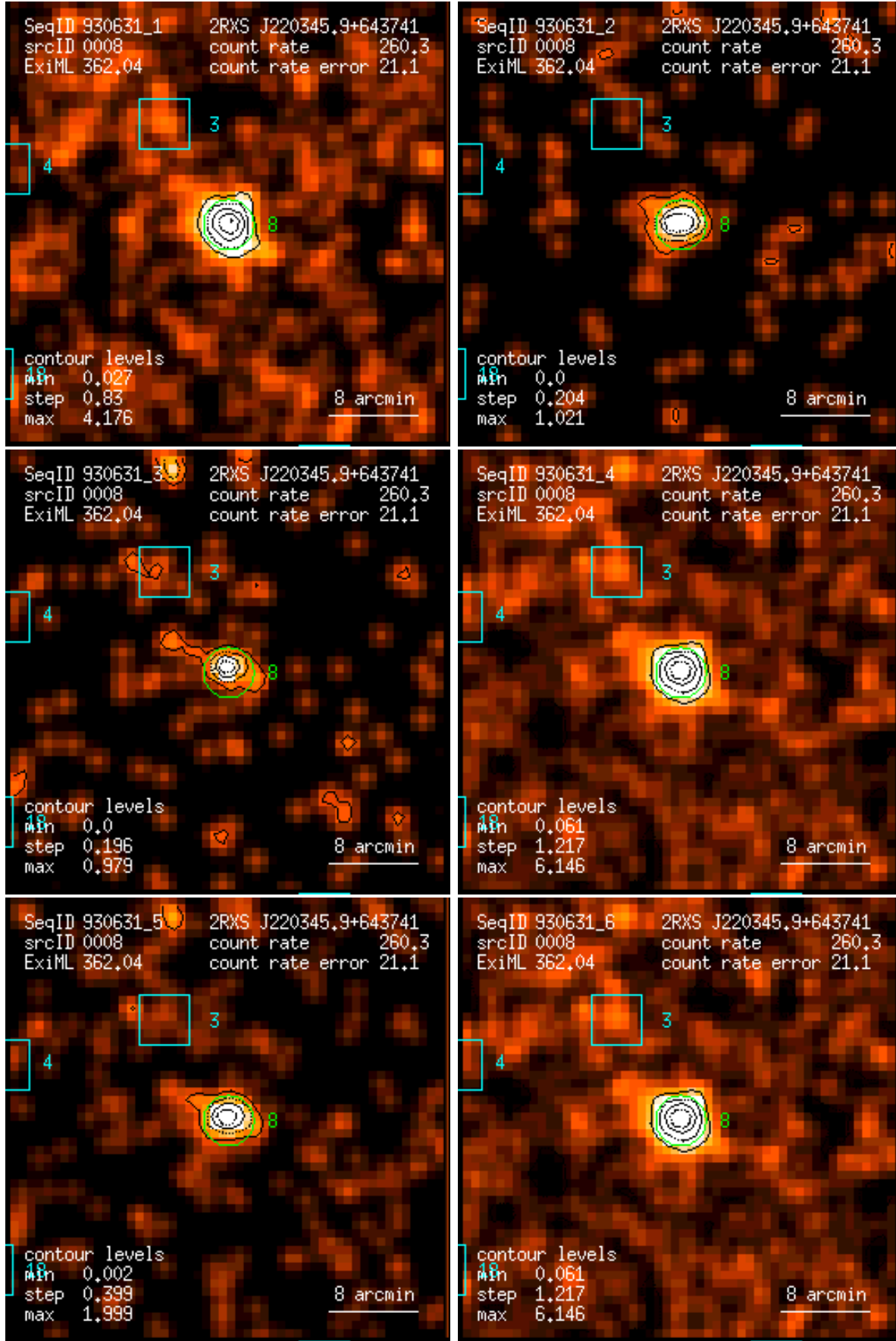
Figure 8: RASS 930631: detection 0008: band rate images, Gaussian filter: (1) PSPC channels 11 – 41, (2) 52 – 90, (3) 91 – 201, (4) 11 – 235, (5) 52 – 201, (6) 11 – 201. Broad band rates in counts/ks. Band rate contour levels in counts/ks/arcmin 2 .
