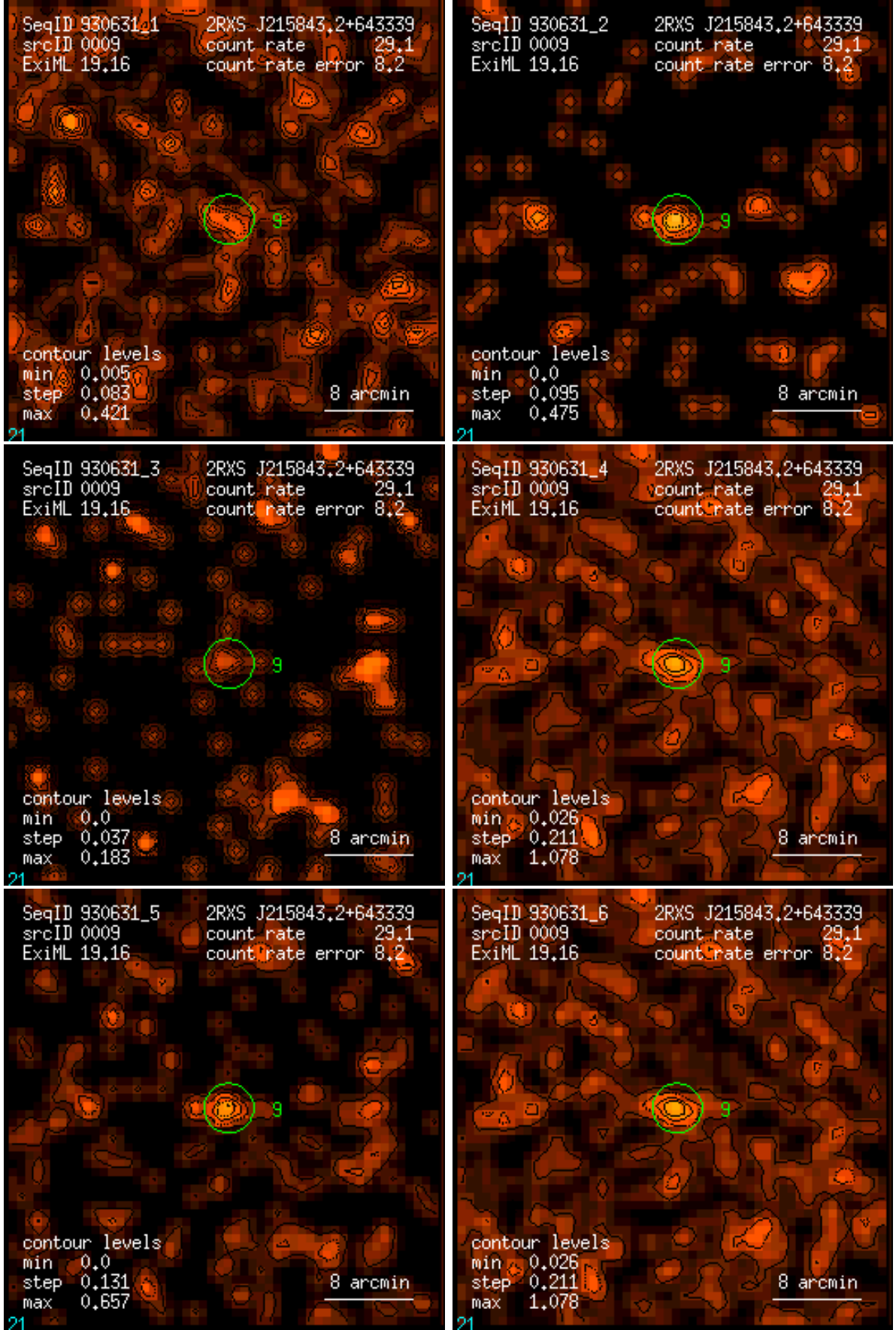
Figure 9: RASS 930631: detection 0009: band rate images, Gaussian filter: (1) PSPC channels 11 – 41, (2) 52 – 90, (3) 91 – 201, (4) 11 – 235, (5) 52 – 201, (6) 11 – 201. Broad band rates in counts/ks. Band rate contour levels in counts/ks/arcmin 2 .
