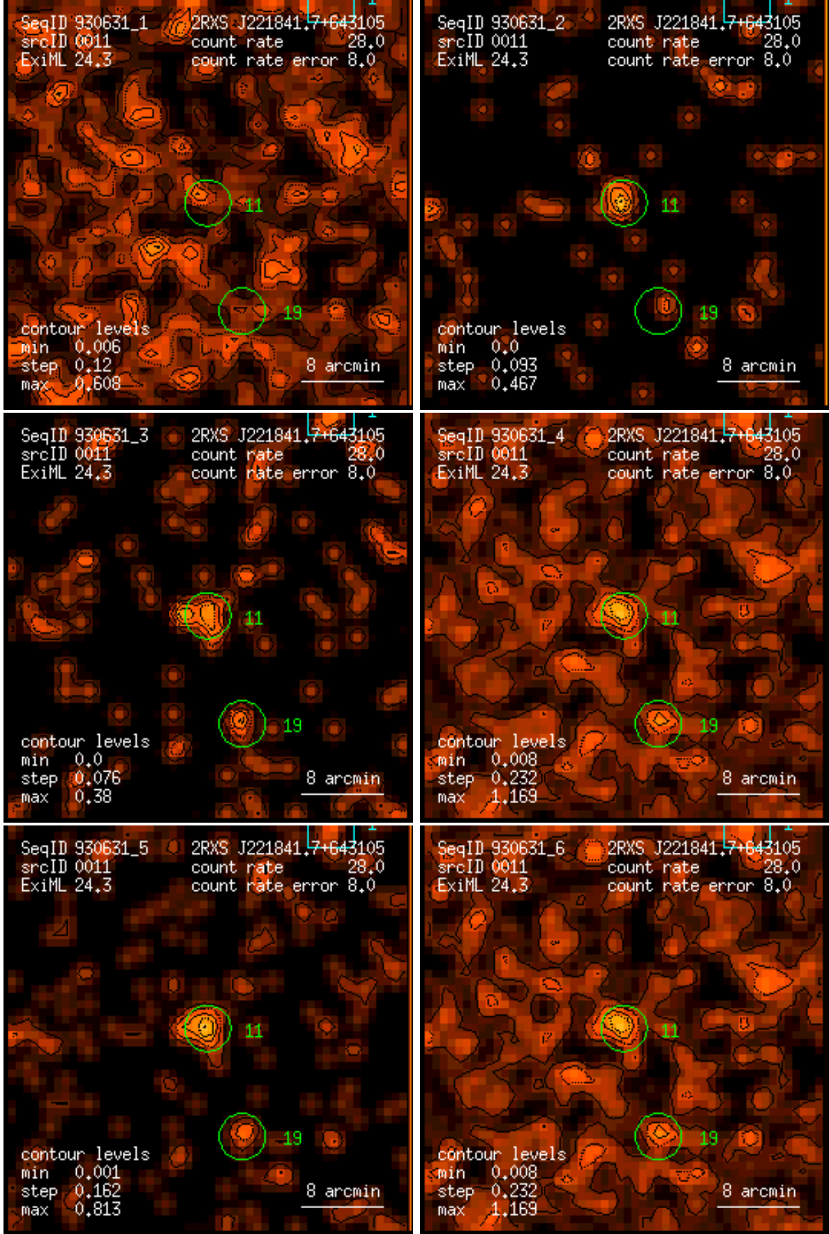
Figure 11: RASS 930631: detection 0011: band rate images, Gaussian filter: (1) PSPC channels 11 – 41, (2) 52 – 90, (3) 91 – 201, (4) 11 – 235, (5) 52 – 201, (6) 11 – 201. Broad band rates in counts/ks. Band rate contour levels in counts/ks/arcmin 2 .
