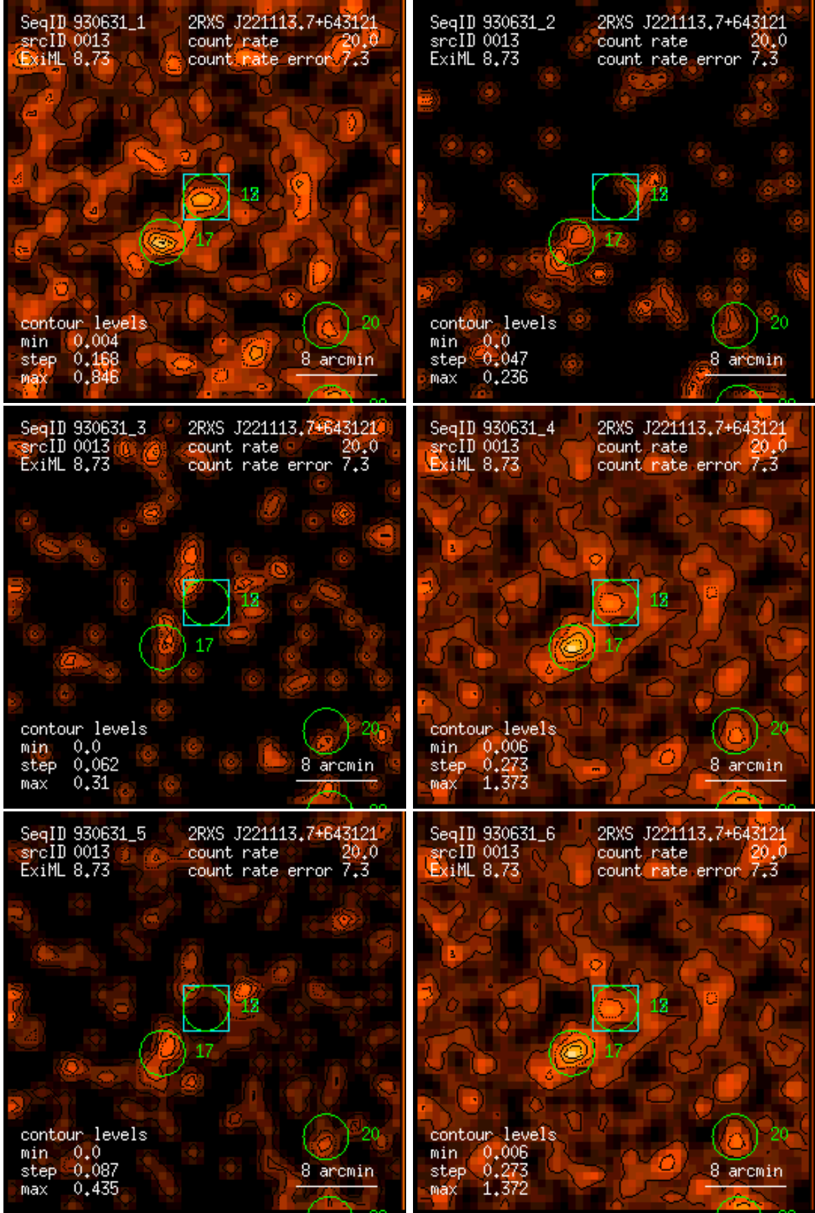
Figure 13: RASS 930631: detection 0013: band rate images, Gaussian filter: (1) PSPC channels 11 – 41, (2) 52 – 90, (3) 91 – 201, (4) 11 – 235, (5) 52 – 201, (6) 11 – 201. Broad band rates in counts/ks. Band rate contour levels in counts/ks/arcmin 2 .
