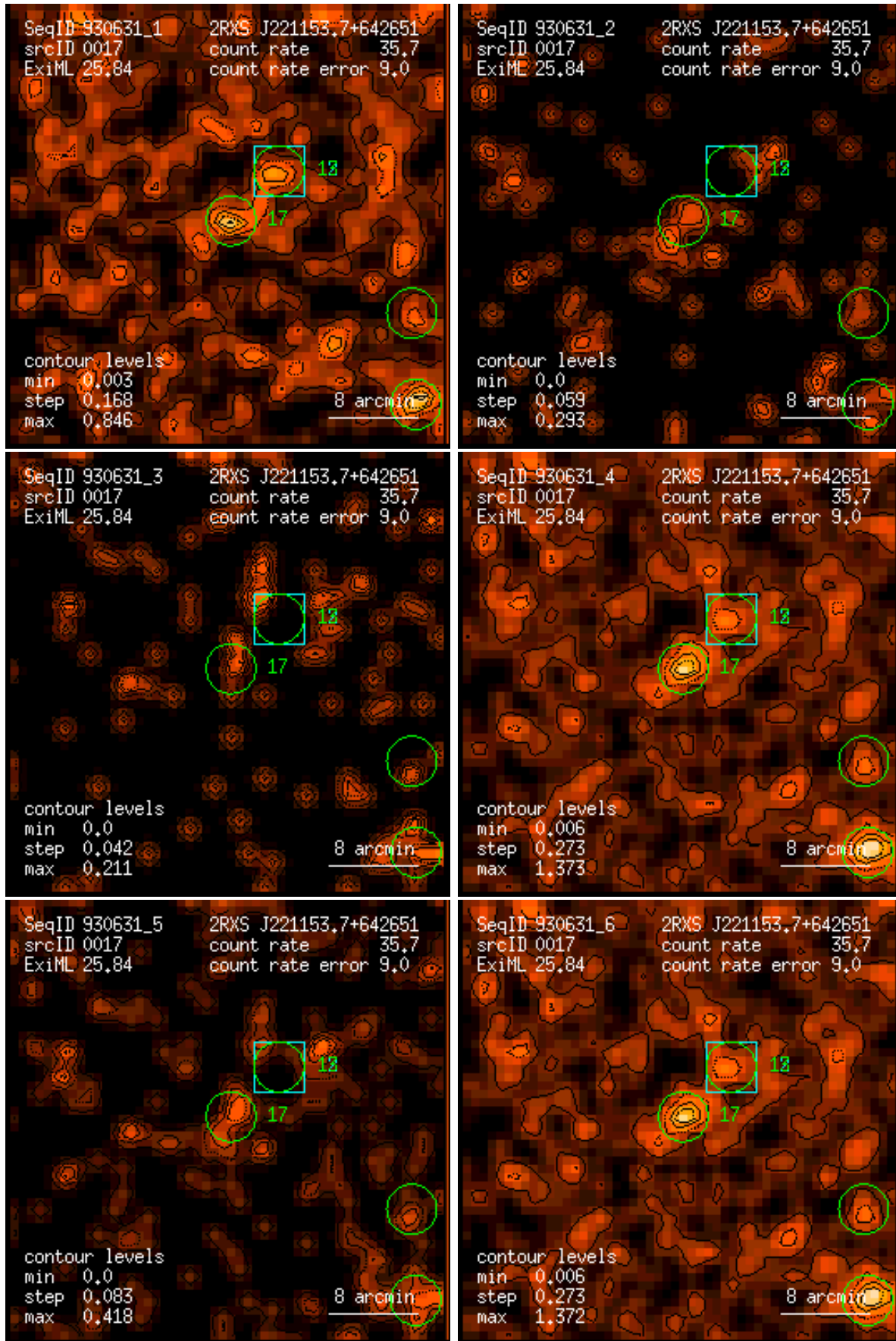
Figure 17: RASS 930631: detection 0017: band rate images, Gaussian filter: (1) PSPC channels 11 – 41, (2) 52 – 90, (3) 91 – 201, (4) 11 – 235, (5) 52 – 201, (6) 11 – 201. Broad band rates in counts/ks. Band rate contour levels in counts/ks/arcmin 2 .
