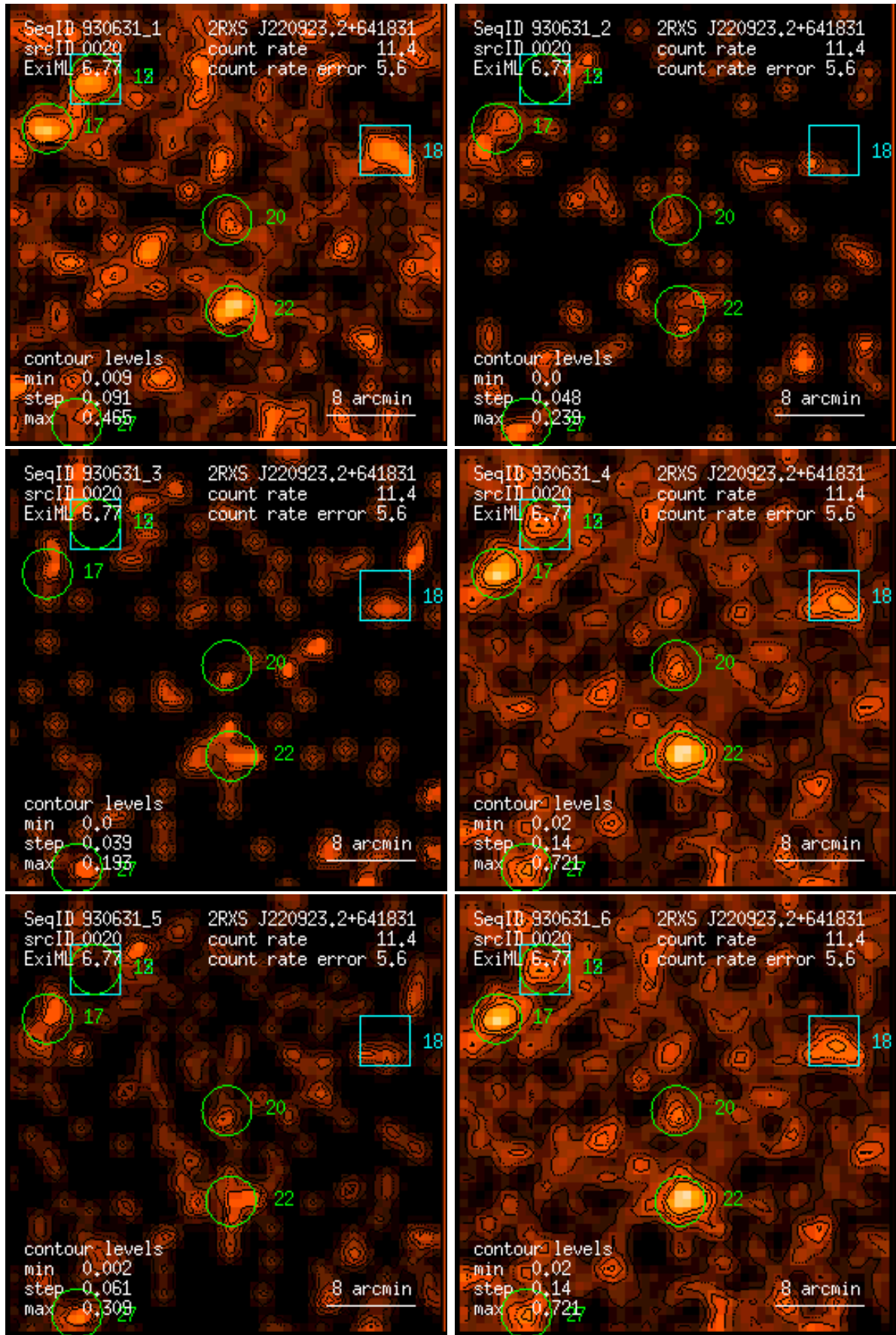
Figure 20: RASS 930631: detection 0020: band rate images, Gaussian filter: (1) PSPC channels 11 – 41, (2) 52 – 90, (3) 91 – 201, (4) 11 – 235, (5) 52 – 201, (6) 11 – 201. Broad band rates in counts/ks. Band rate contour levels in counts/ks/arcmin 2 .
