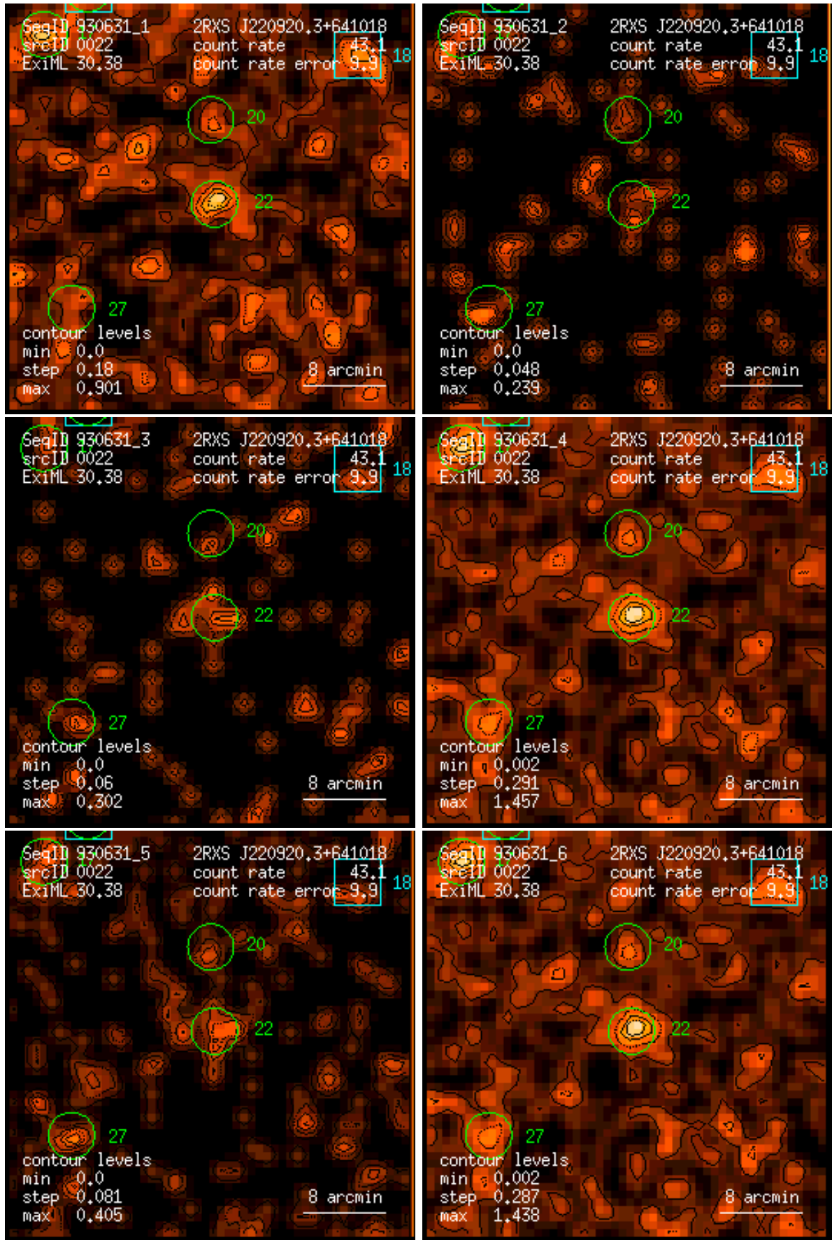
Figure 22: RASS 930631: detection 0022: band rate images, Gaussian filter: (1) PSPC channels 11 – 41, (2) 52 – 90, (3) 91 – 201, (4) 11 – 235, (5) 52 – 201, (6) 11 – 201. Broad band rates in counts/ks. Band rate contour levels in counts/ks/arcmin 2 .
