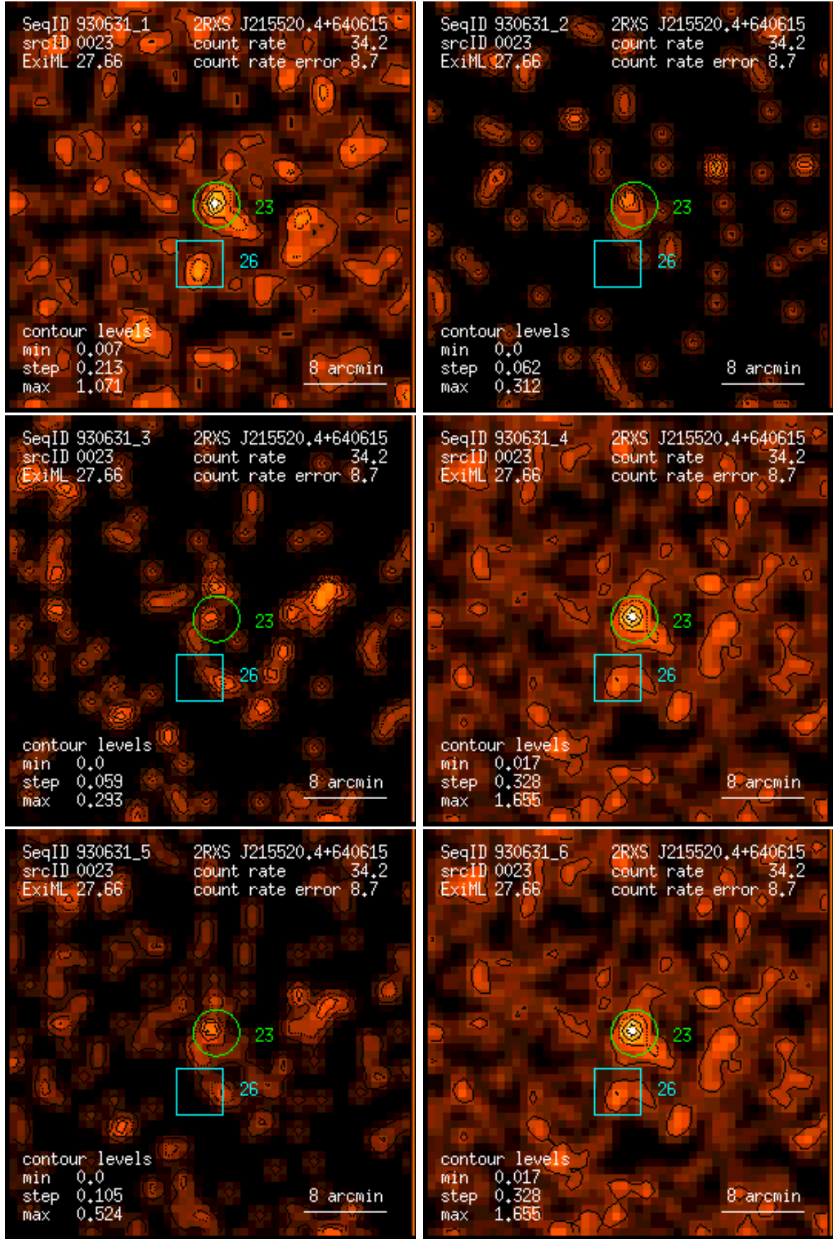
Figure 23: RASS 930631: detection 0023: band rate images, Gaussian filter: (1) PSPC channels 11 – 41, (2) 52 – 90, (3) 91 – 201, (4) 11 – 235, (5) 52 – 201, (6) 11 – 201. Broad band rates in counts/ks. Band rate contour levels in counts/ks/arcmin 2 .
