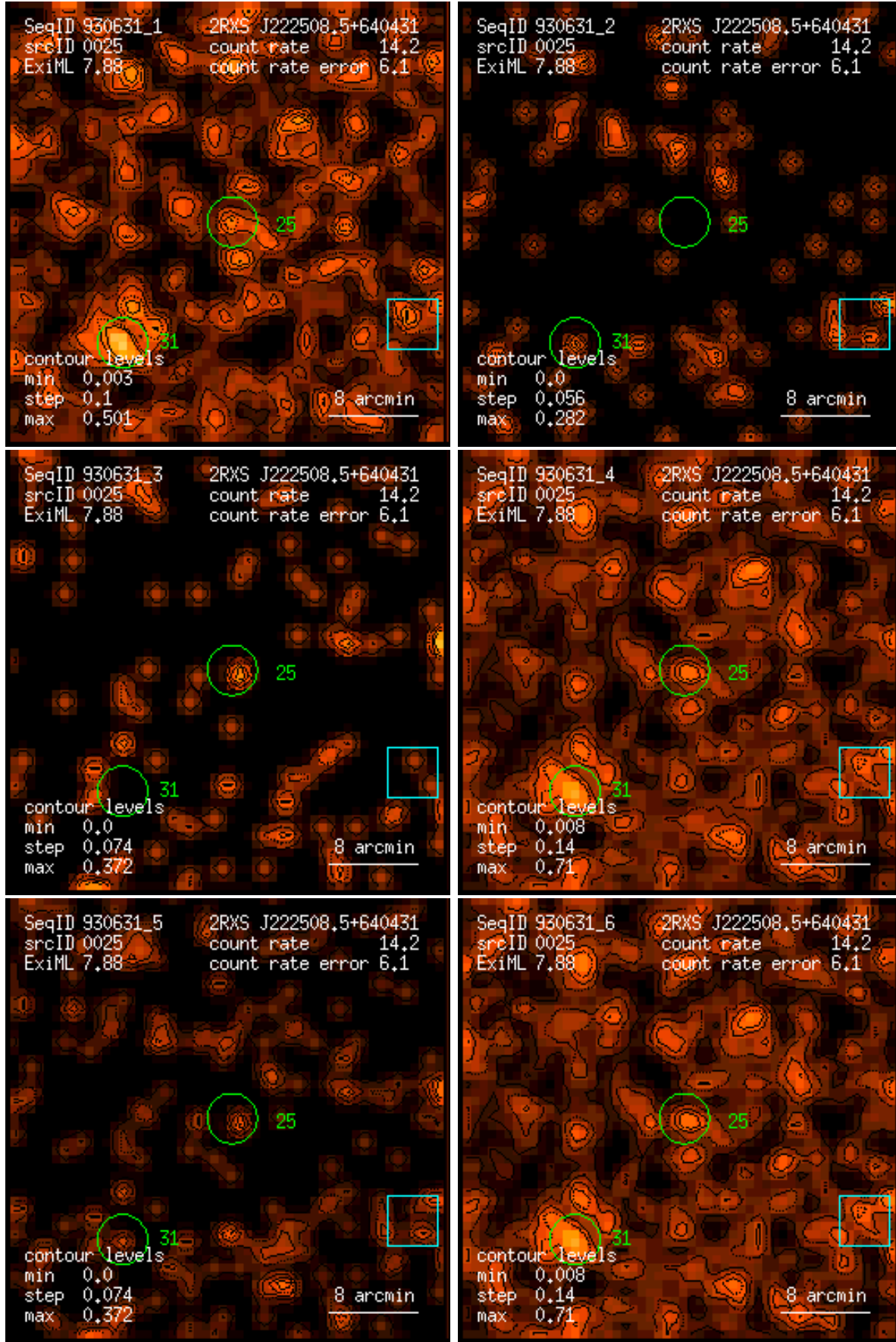
Figure 25: RASS 930631: detection 0025: band rate images, Gaussian filter: (1) PSPC channels 11 – 41, (2) 52 – 90, (3) 91 – 201, (4) 11 – 235, (5) 52 – 201, (6) 11 – 201. Broad band rates in counts/ks. Band rate contour levels in counts/ks/arcmin 2 .
