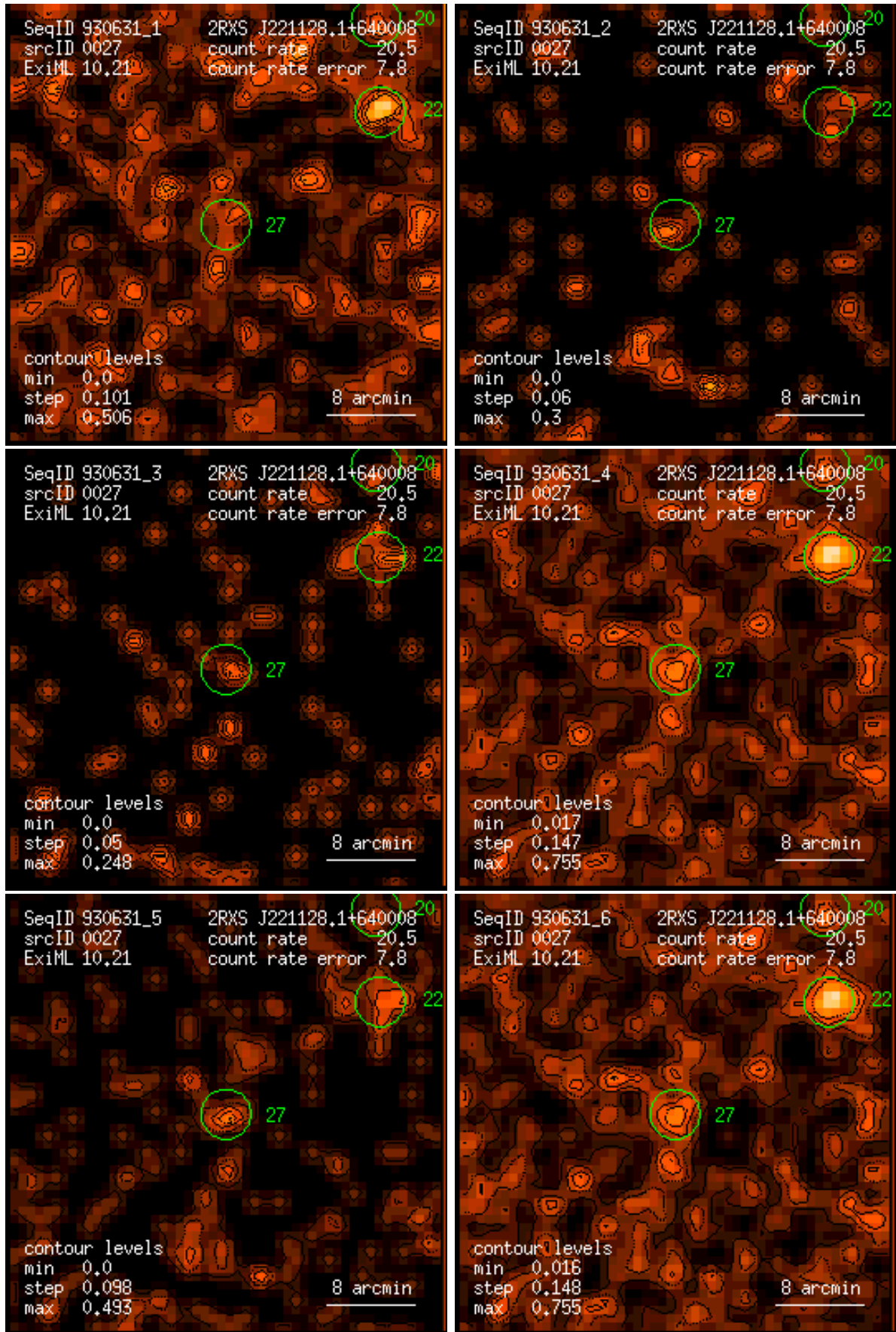
Figure 27: RASS 930631: detection 0027: band rate images, Gaussian filter: (1) PSPC channels 11 – 41, (2) 52 – 90, (3) 91 – 201, (4) 11 – 235, (5) 52 – 201, (6) 11 – 201. Broad band rates in counts/ks. Band rate contour levels in counts/ks/arcmin 2 .
