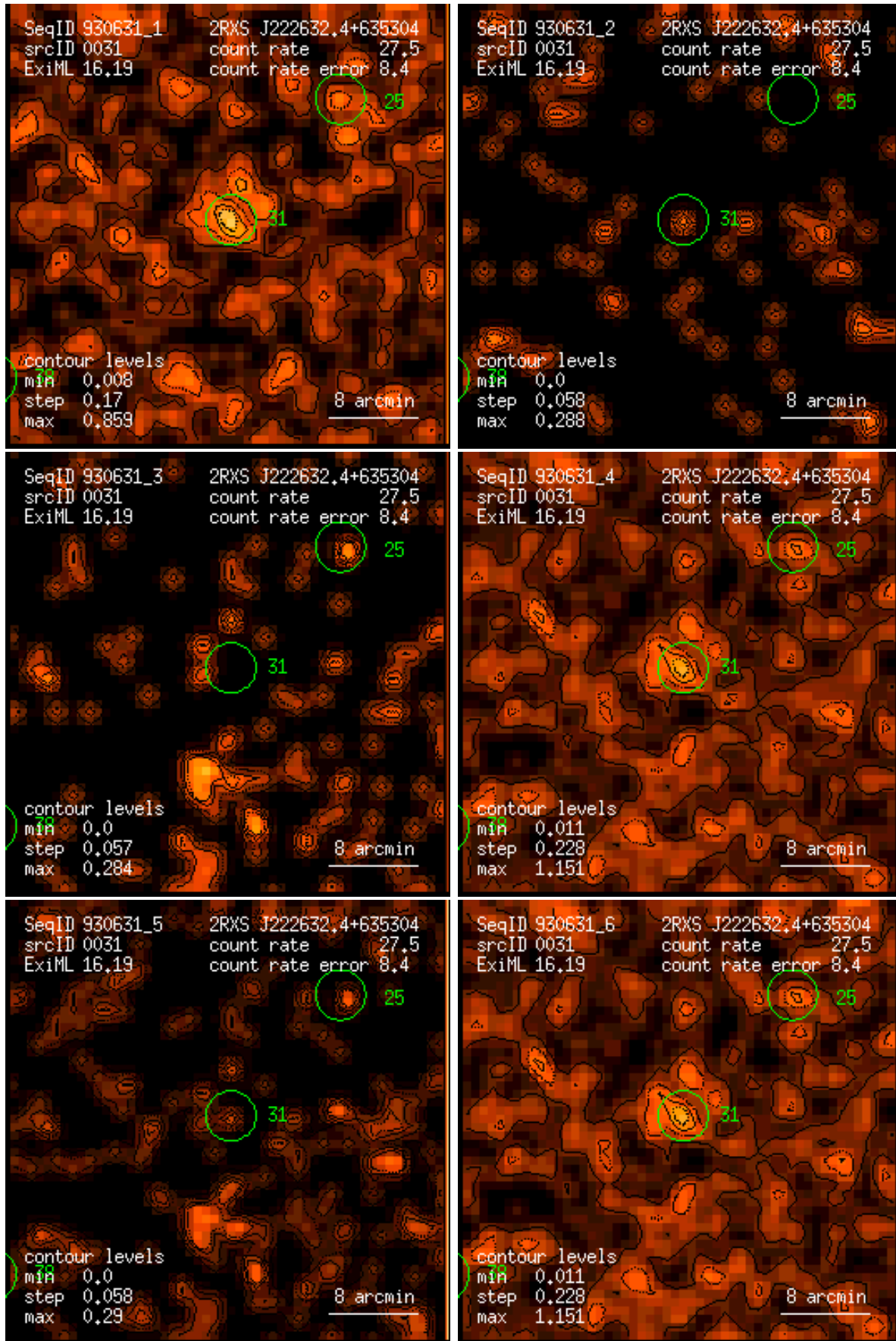
Figure 31: RASS 930631: detection 0031: band rate images, Gaussian filter: (1) PSPC channels 11 – 41, (2) 52 – 90, (3) 91 – 201, (4) 11 – 235, (5) 52 – 201, (6) 11 – 201. Broad band rates in counts/ks. Band rate contour levels in counts/ks/arcmin 2 .
