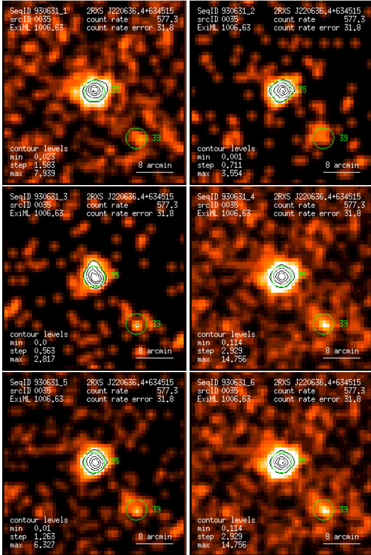
Figure 35: RASS 930631: detection 0035: band rate images, Gaussian filter: (1) PSPC channels 11 – 41, (2) 52 – 90, (3) 91 – 201, (4) 11 – 235, (5) 52 – 201, (6) 11 – 201. Broad band rates in counts/ks. Band rate contour levels in counts/ks/arcmin 2 .
