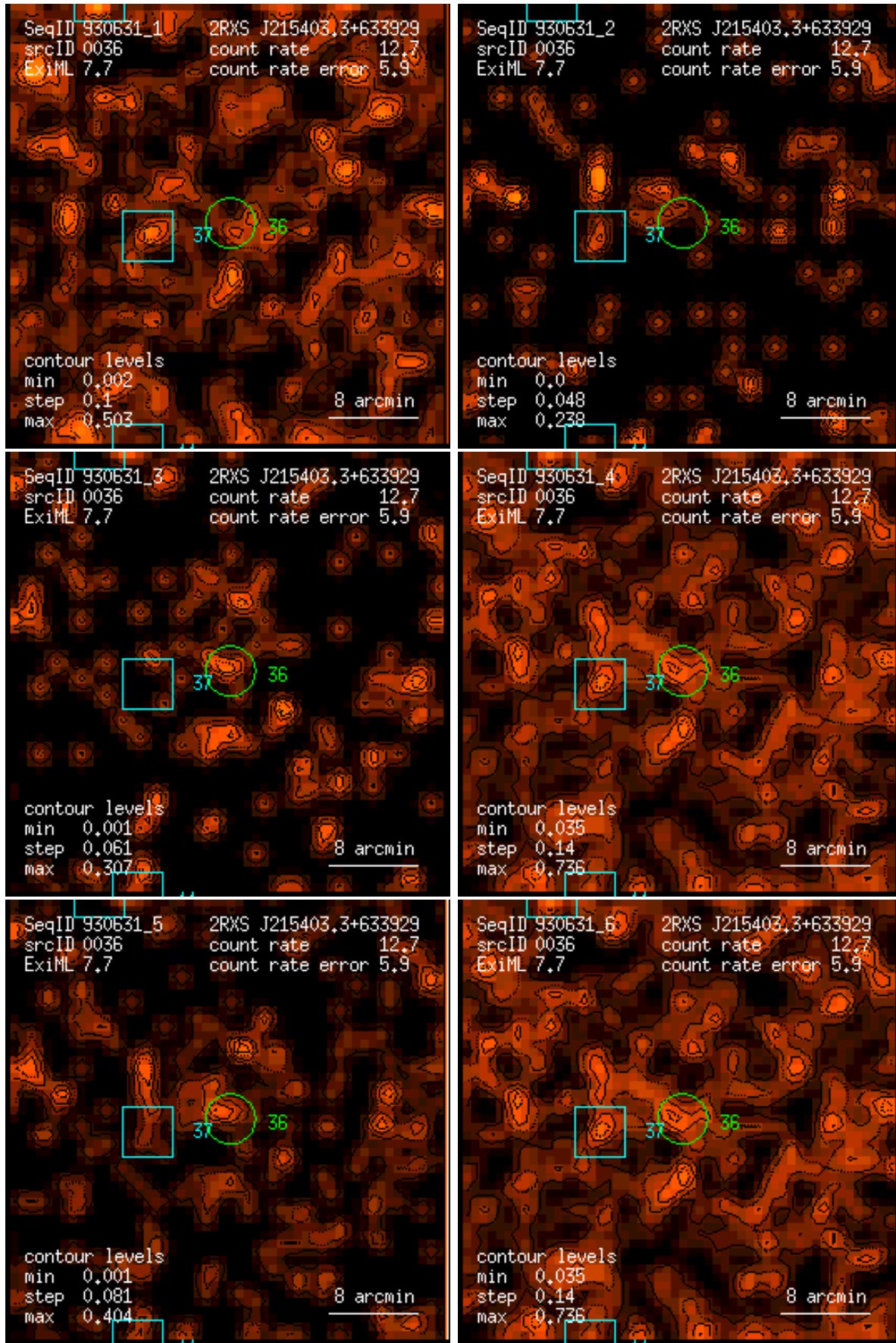
Figure 36: RASS 930631: detection 0036: band rate images, Gaussian filter: (1) PSPC channels 11 – 41, (2) 52 – 90, (3) 91 – 201, (4) 11 – 235, (5) 52 – 201, (6) 11 – 201. Broad band rates in counts/ks. Band rate contour levels in counts/ks/arcmin 2 .
