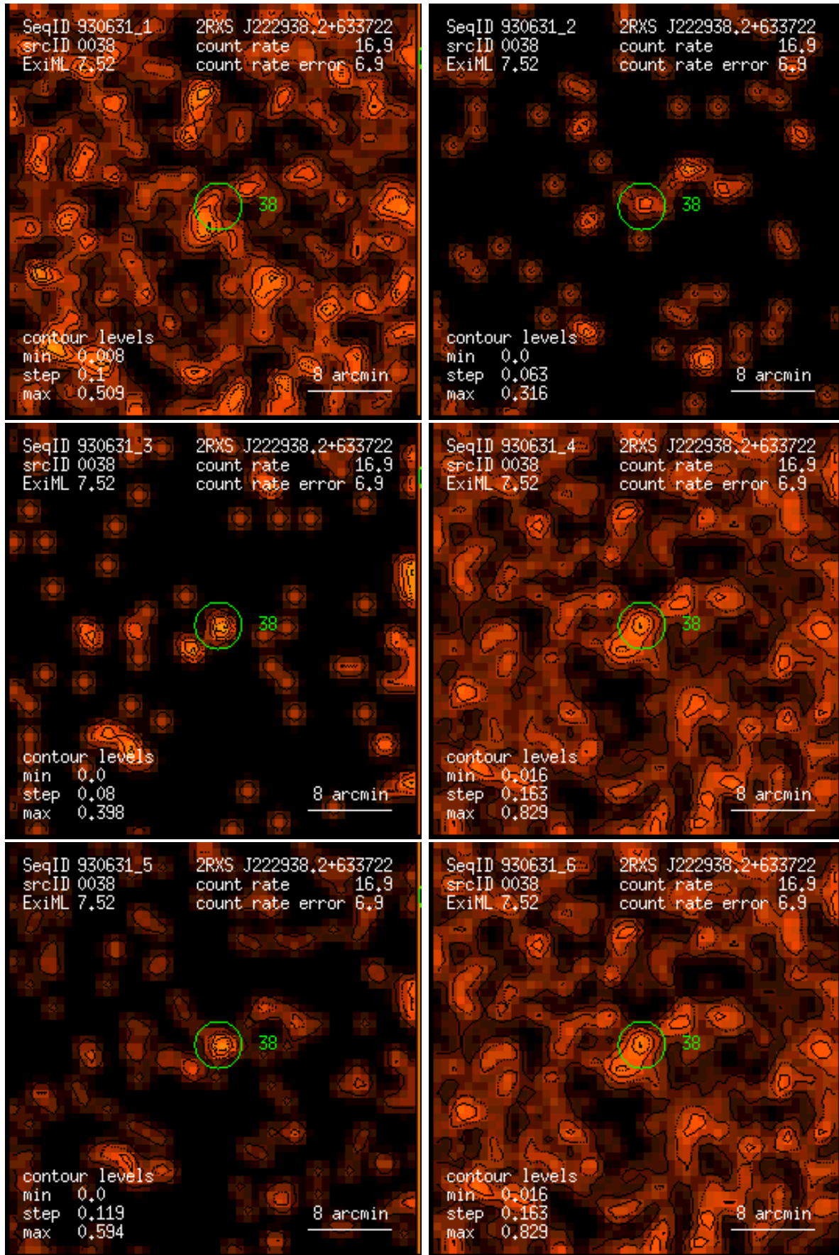
Figure 38: RASS 930631: detection 0038: band rate images, Gaussian filter: (1) PSPC channels 11 – 41, (2) 52 – 90, (3) 91 – 201, (4) 11 – 235, (5) 52 – 201, (6) 11 – 201. Broad band rates in counts/ks. Band rate contour levels in counts/ks/arcmin 2 .
