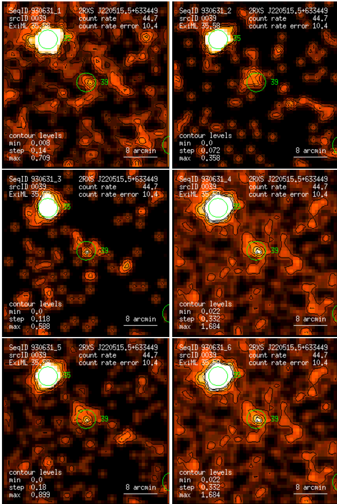
Figure 39: RASS 930631: detection 0039: band rate images, Gaussian filter: (1) PSPC channels 11 – 41, (2) 52 – 90, (3) 91 – 201, (4) 11 – 235, (5) 52 – 201, (6) 11 – 201. Broad band rates in counts/ks. Band rate contour levels in counts/ks/arcmin 2 .
