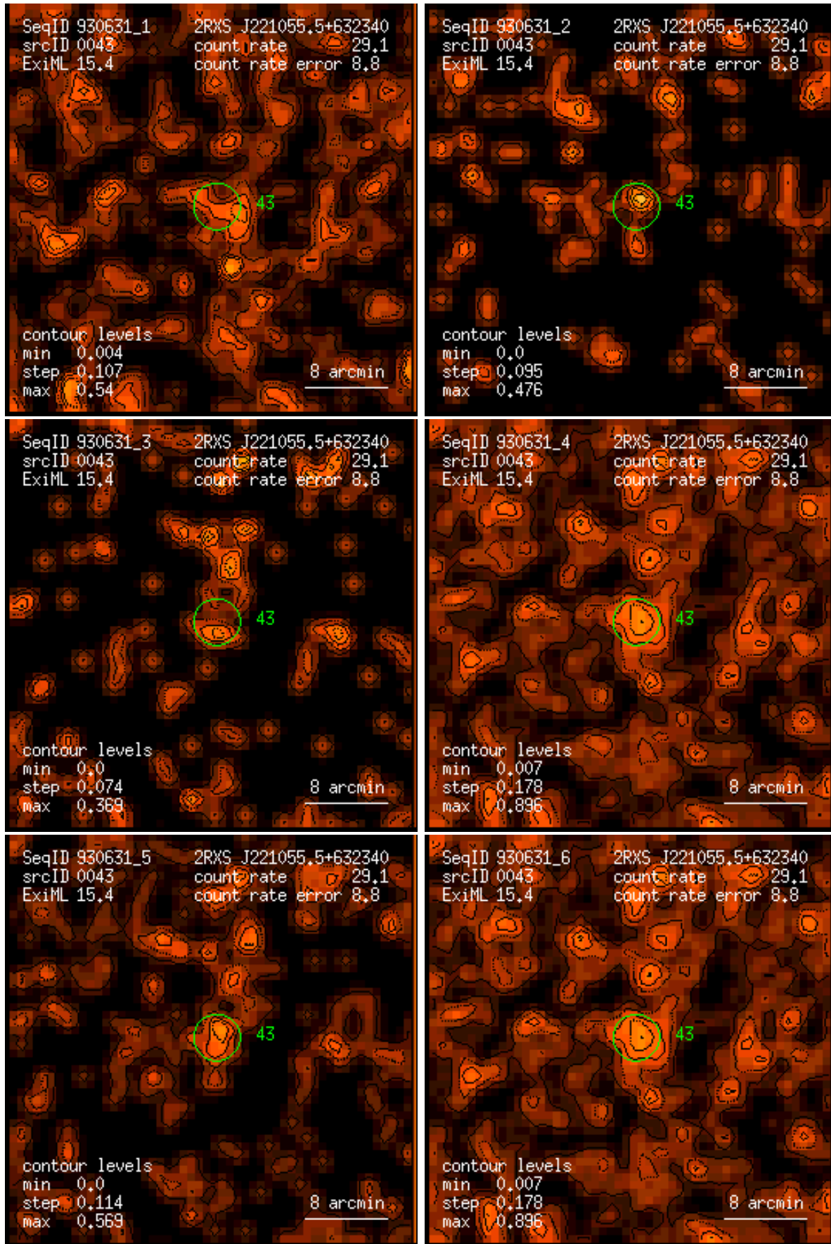
Figure 43: RASS 930631: detection 0043: band rate images, Gaussian filter: (1) PSPC channels 11 – 41, (2) 52 – 90, (3) 91 – 201, (4) 11 – 235, (5) 52 – 201, (6) 11 – 201. Broad band rates in counts/ks. Band rate contour levels in counts/ks/arcmin 2 .
