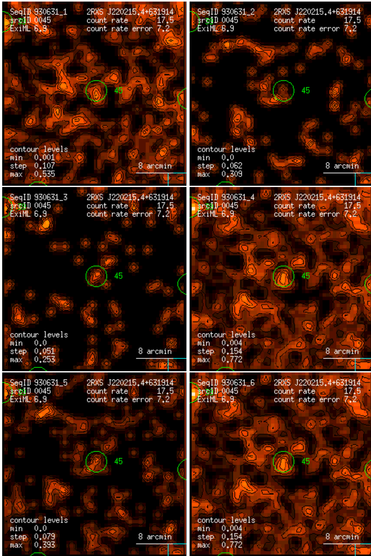
Figure 45: RASS 930631: detection 0045: band rate images, Gaussian filter: (1) PSPC channels 11 – 41, (2) 52 – 90, (3) 91 – 201, (4) 11 – 235, (5) 52 – 201, (6) 11 – 201. Broad band rates in counts/ks. Band rate contour levels in counts/ks/arcmin 2 .
