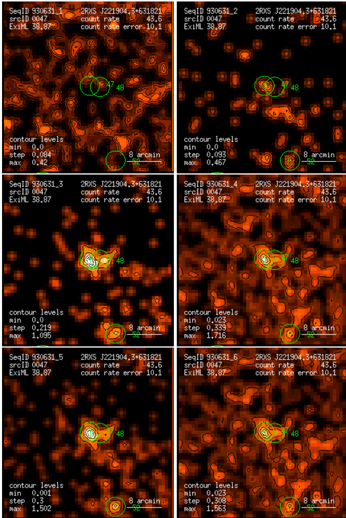
Figure 47: RASS 930631: detection 0047: band rate images, Gaussian filter: (1) PSPC channels 11 – 41, (2) 52 – 90, (3) 91 – 201, (4) 11 – 235, (5) 52 – 201, (6) 11 – 201. Broad band rates in counts/ks. Band rate contour levels in counts/ks/arcmin 2 .
