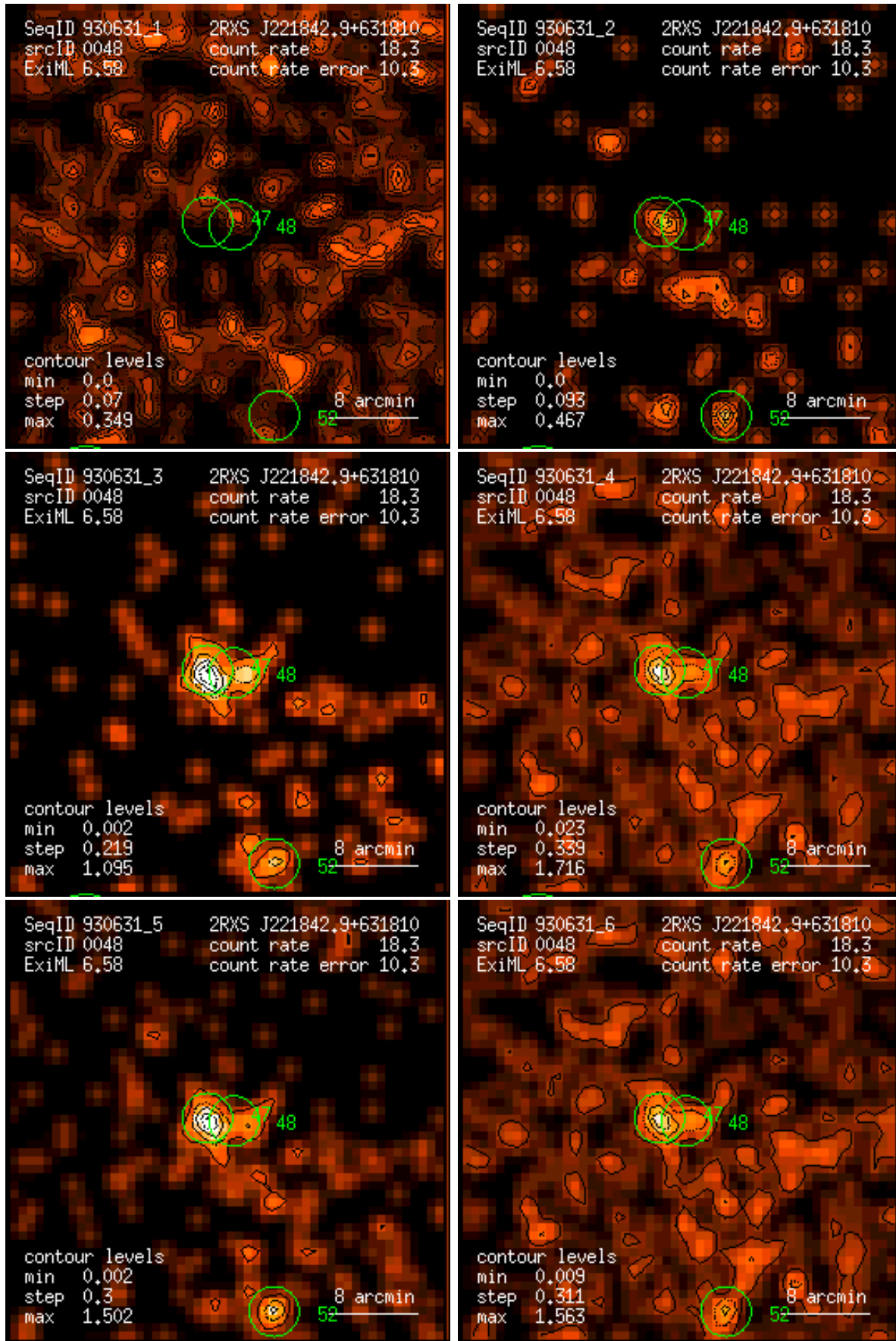
Figure 48: RASS 930631: detection 0048: band rate images, Gaussian filter: (1) PSPC channels 11 – 41, (2) 52 – 90, (3) 91 – 201, (4) 11 – 235, (5) 52 – 201, (6) 11 – 201. Broad band rates in counts/ks. Band rate contour levels in counts/ks/arcmin 2 .
