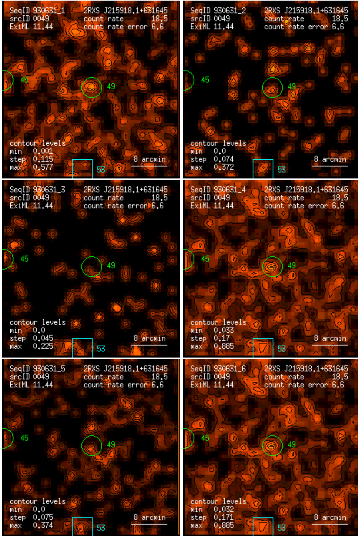
Figure 49: RASS 930631: detection 0049: band rate images, Gaussian filter: (1) PSPC channels 11 – 41, (2) 52 – 90, (3) 91 – 201, (4) 11 – 235, (5) 52 – 201, (6) 11 – 201. Broad band rates in counts/ks. Band rate contour levels in counts/ks/arcmin 2 .
