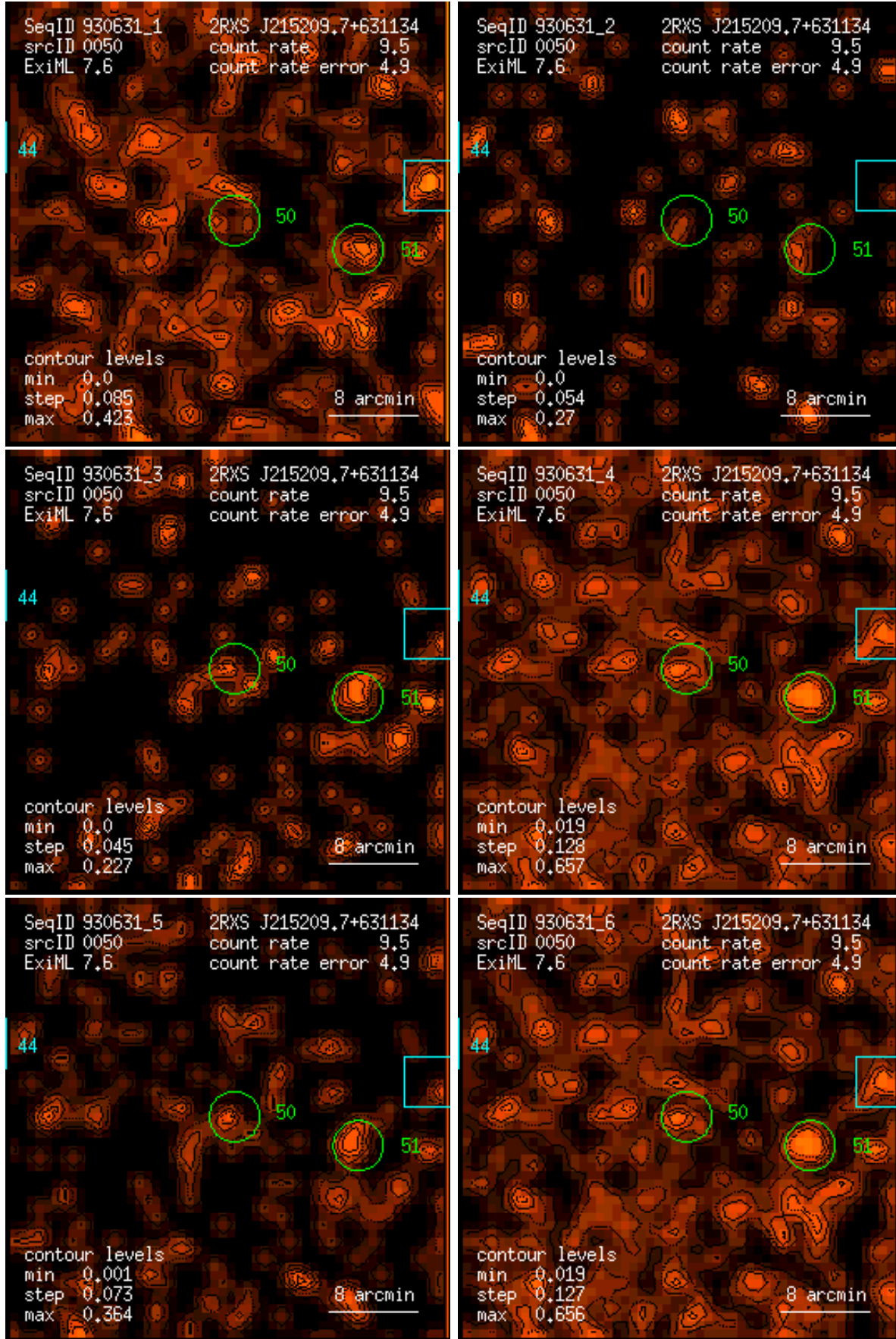
Figure 50: RASS 930631: detection 0050: band rate images, Gaussian filter: (1) PSPC channels 11 – 41, (2) 52 – 90, (3) 91 – 201, (4) 11 – 235, (5) 52 – 201, (6) 11 – 201. Broad band rates in counts/ks. Band rate contour levels in counts/ks/arcmin 2 .
