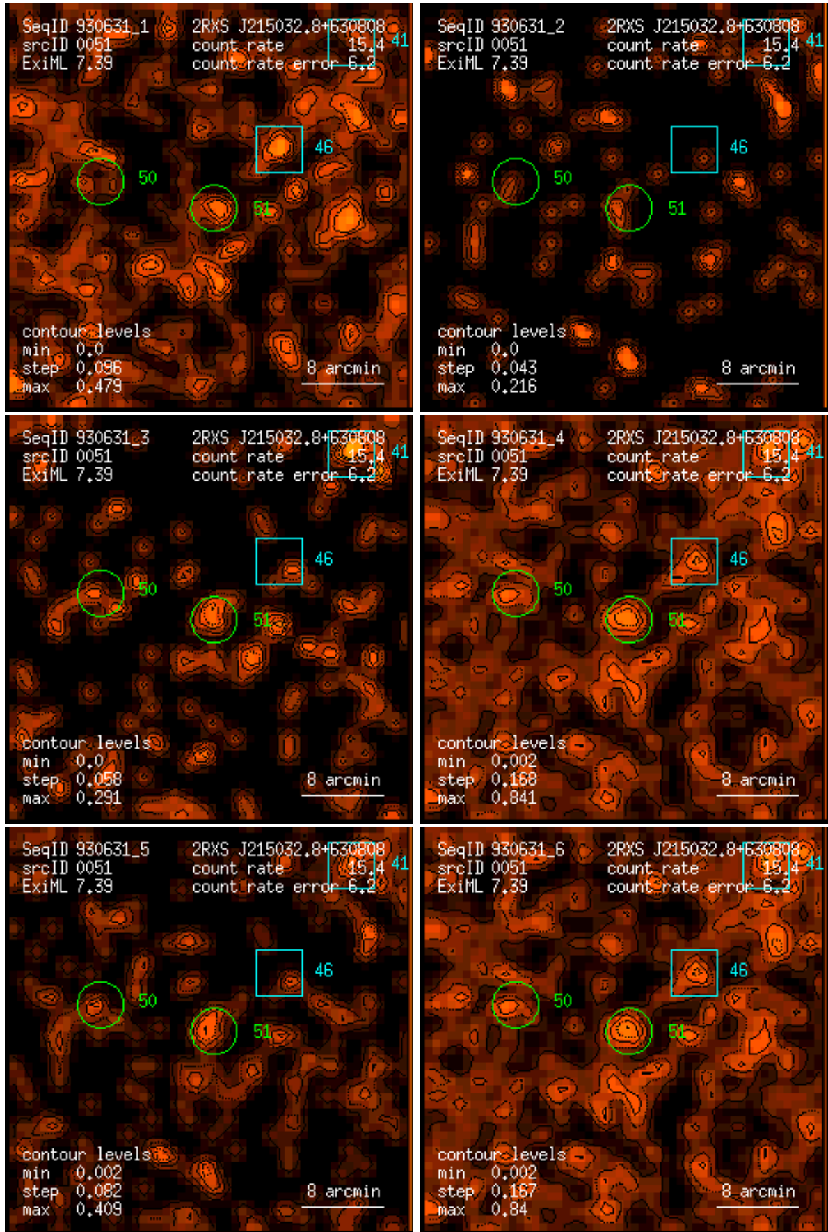
Figure 51: RASS 930631: detection 0051: band rate images, Gaussian filter: (1) PSPC channels 11 – 41, (2) 52 – 90, (3) 91 – 201, (4) 11 – 235, (5) 52 – 201, (6) 11 – 201. Broad band rates in counts/ks. Band rate contour levels in counts/ks/arcmin 2 .
