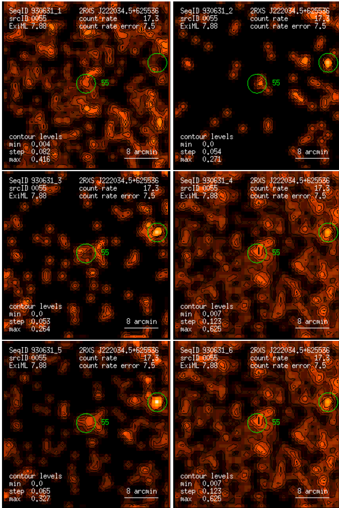
Figure 55: RASS 930631: detection 0055: band rate images, Gaussian filter: (1) PSPC channels 11 – 41, (2) 52 – 90, (3) 91 – 201, (4) 11 – 235, (5) 52 – 201, (6) 11 – 201. Broad band rates in counts/ks. Band rate contour levels in counts/ks/arcmin 2 .
