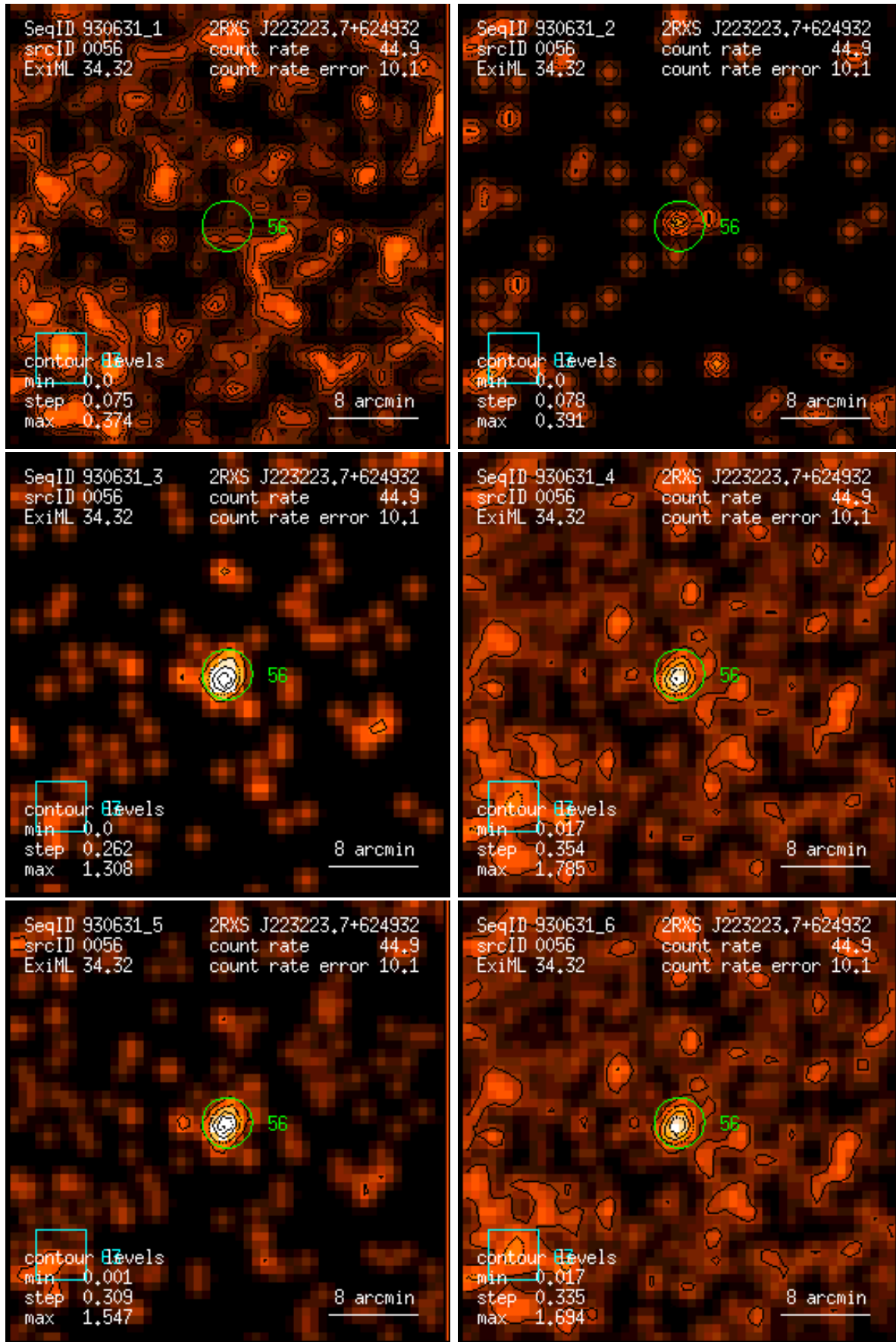
Figure 56: RASS 930631: detection 0056: band rate images, Gaussian filter: (1) PSPC channels 11 – 41, (2) 52 – 90, (3) 91 – 201, (4) 11 – 235, (5) 52 – 201, (6) 11 – 201. Broad band rates in counts/ks. Band rate contour levels in counts/ks/arcmin 2 .
