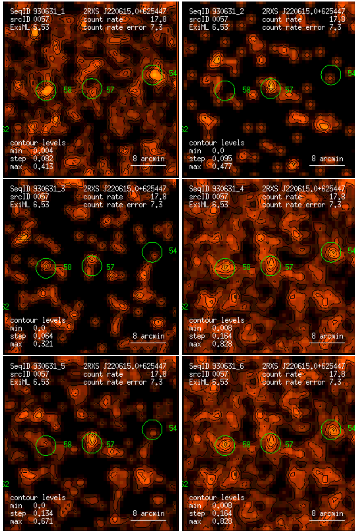
Figure 57: RASS 930631: detection 0057: band rate images, Gaussian filter: (1) PSPC channels 11 – 41, (2) 52 – 90, (3) 91 – 201, (4) 11 – 235, (5) 52 – 201, (6) 11 – 201. Broad band rates in counts/ks. Band rate contour levels in counts/ks/arcmin 2 .
