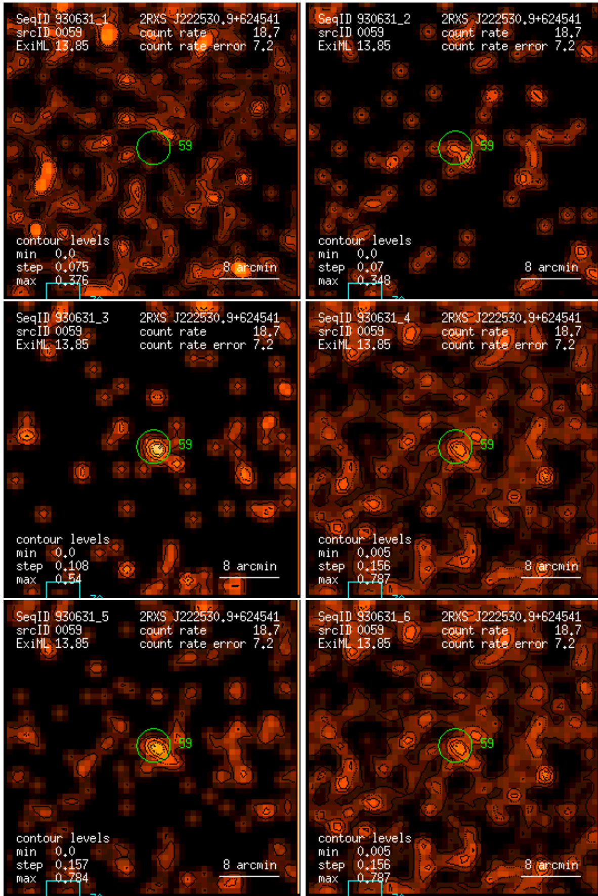
Figure 59: RASS 930631: detection 0059: band rate images, Gaussian filter: (1) PSPC channels 11 – 41, (2) 52 – 90, (3) 91 – 201, (4) 11 – 235, (5) 52 – 201, (6) 11 – 201. Broad band rates in counts/ks. Band rate contour levels in counts/ks/arcmin 2 .
