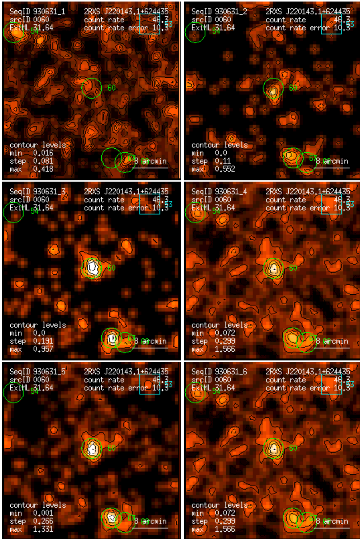
Figure 60: RASS 930631: detection 0060: band rate images, Gaussian filter: (1) PSPC channels 11 – 41, (2) 52 – 90, (3) 91 – 201, (4) 11 – 235, (5) 52 – 201, (6) 11 – 201. Broad band rates in counts/ks. Band rate contour levels in counts/ks/arcmin 2 .
