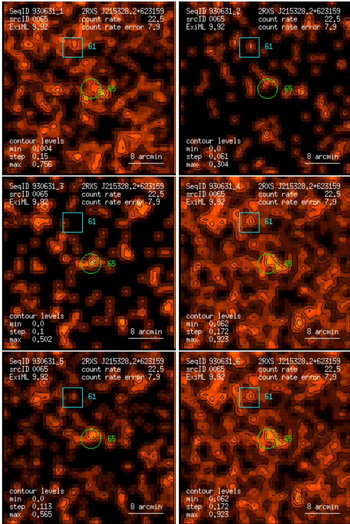
Figure 65: RASS 930631: detection 0065: band rate images, Gaussian filter: (1) PSPC channels 11 – 41, (2) 52 – 90, (3) 91 – 201, (4) 11 – 235, (5) 52 – 201, (6) 11 – 201. Broad band rates in counts/ks. Band rate contour levels in counts/ks/arcmin 2 .
