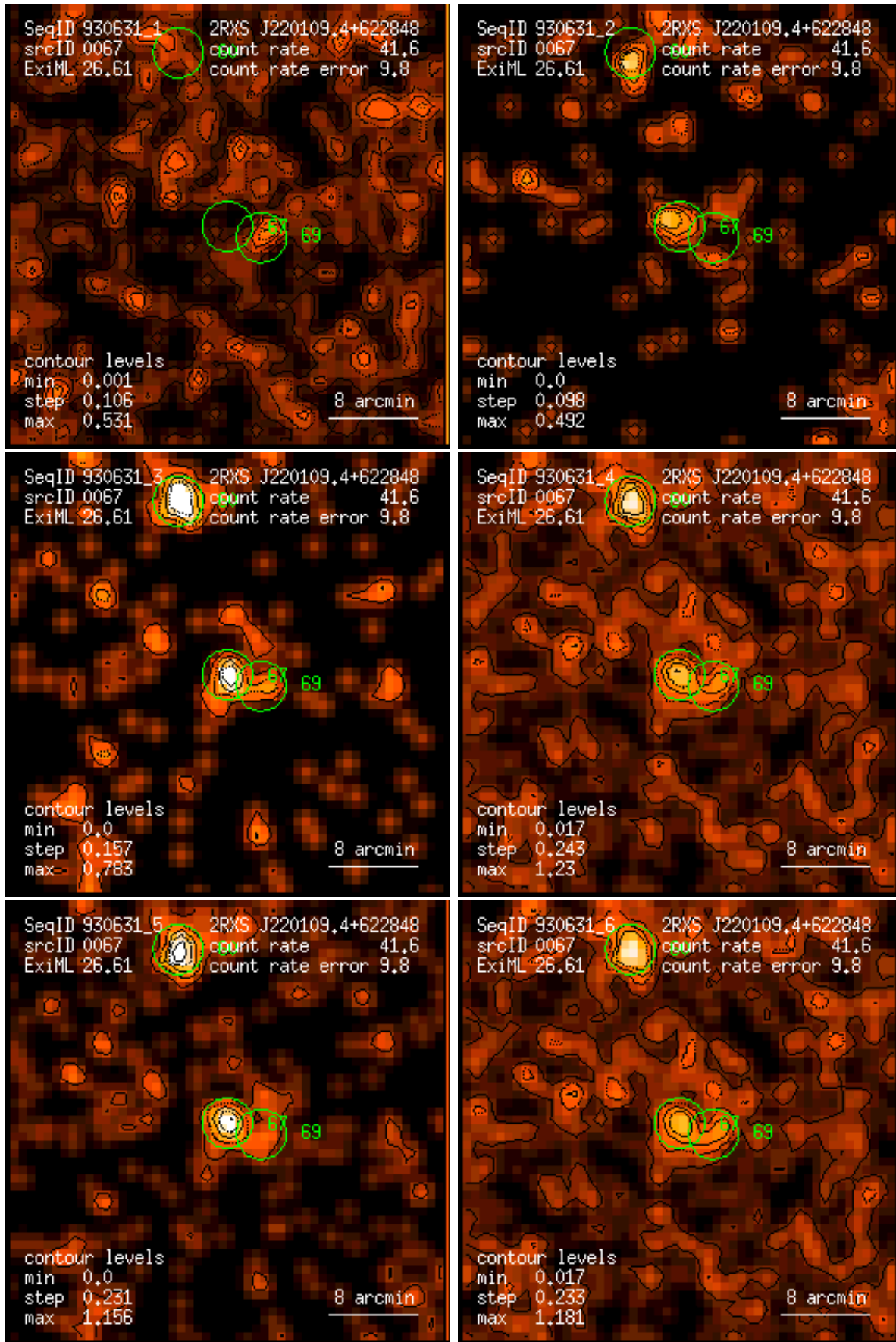
Figure 67: RASS 930631: detection 0067: band rate images, Gaussian filter: (1) PSPC channels 11 – 41, (2) 52 – 90, (3) 91 – 201, (4) 11 – 235, (5) 52 – 201, (6) 11 – 201. Broad band rates in counts/ks. Band rate contour levels in counts/ks/arcmin 2 .
