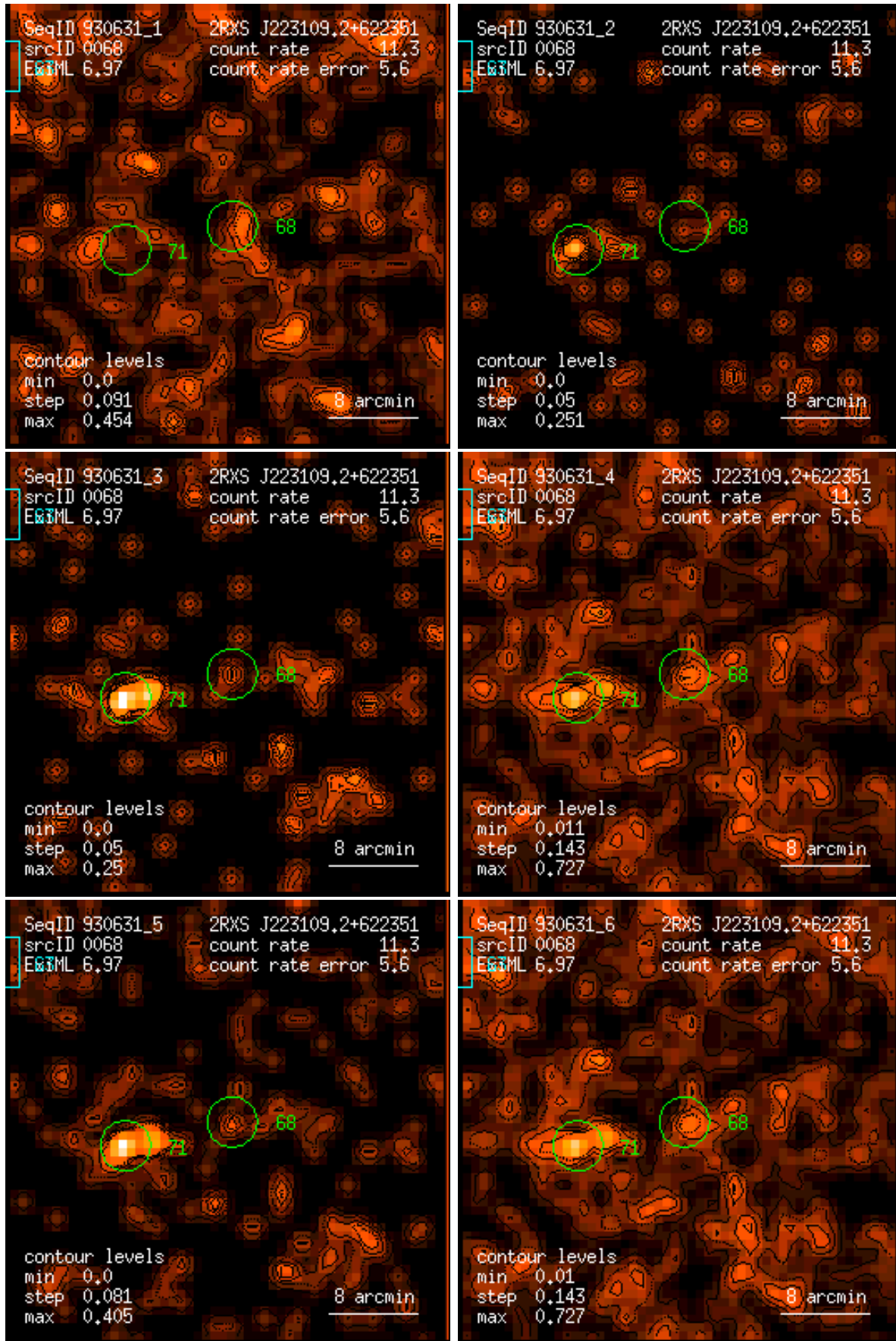
Figure 68: RASS 930631: detection 0068: band rate images, Gaussian filter: (1) PSPC channels 11 – 41, (2) 52 – 90, (3) 91 – 201, (4) 11 – 235, (5) 52 – 201, (6) 11 – 201. Broad band rates in counts/ks. Band rate contour levels in counts/ks/arcmin 2 .
