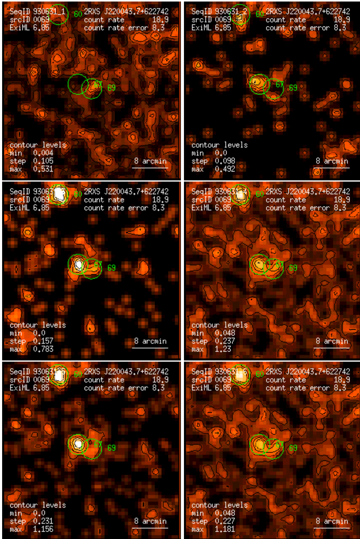
Figure 69: RASS 930631: detection 0069: band rate images, Gaussian filter: (1) PSPC channels 11 – 41, (2) 52 – 90, (3) 91 – 201, (4) 11 – 235, (5) 52 – 201, (6) 11 – 201. Broad band rates in counts/ks. Band rate contour levels in counts/ks/arcmin 2 .
