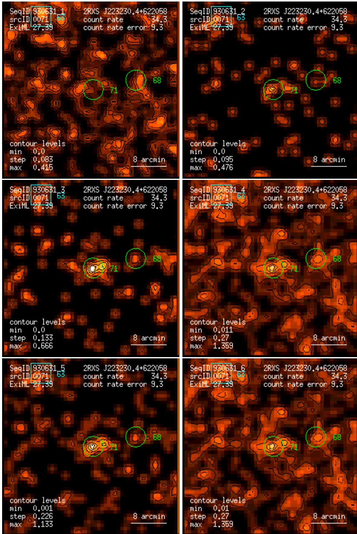
Figure 71: RASS 930631: detection 0071: band rate images, Gaussian filter: (1) PSPC channels 11 – 41, (2) 52 – 90, (3) 91 – 201, (4) 11 – 235, (5) 52 – 201, (6) 11 – 201. Broad band rates in counts/ks. Band rate contour levels in counts/ks/arcmin 2 .
