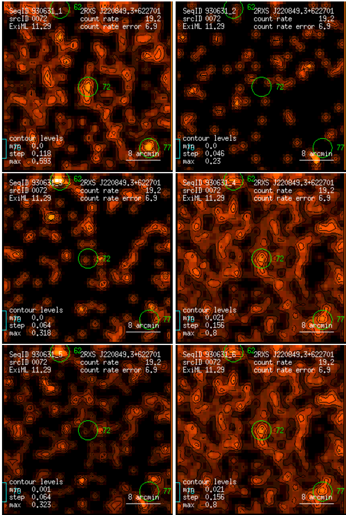
Figure 72: RASS 930631: detection 0072: band rate images, Gaussian filter: (1) PSPC channels 11 – 41, (2) 52 – 90, (3) 91 – 201, (4) 11 – 235, (5) 52 – 201, (6) 11 – 201. Broad band rates in counts/ks. Band rate contour levels in counts/ks/arcmin 2 .
