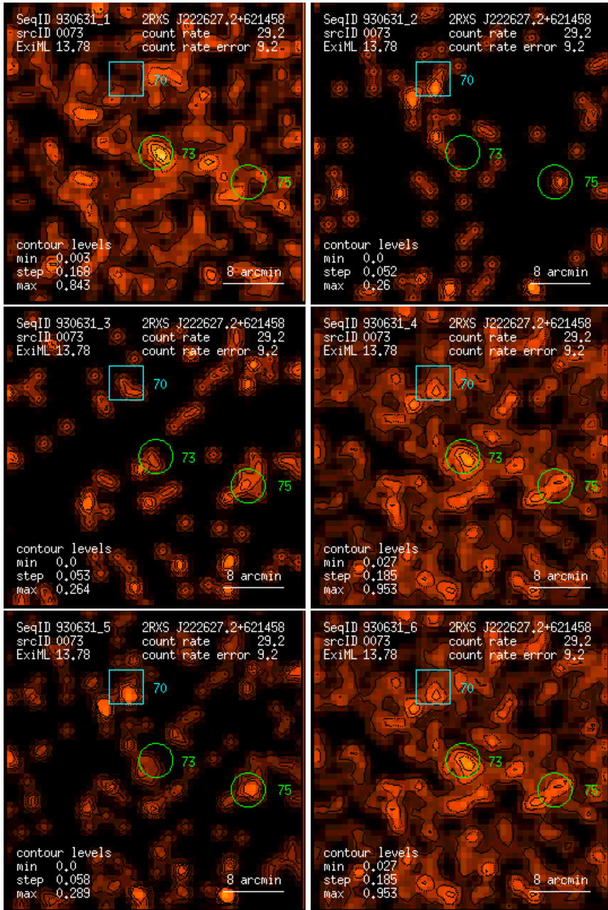
Figure 73: RASS 930631: detection 0073: band rate images, Gaussian filter: (1) PSPC channels 11 – 41, (2) 52 – 90, (3) 91 – 201, (4) 11 – 235, (5) 52 – 201, (6) 11 – 201. Broad band rates in counts/ks. Band rate contour levels in counts/ks/arcmin 2 .
