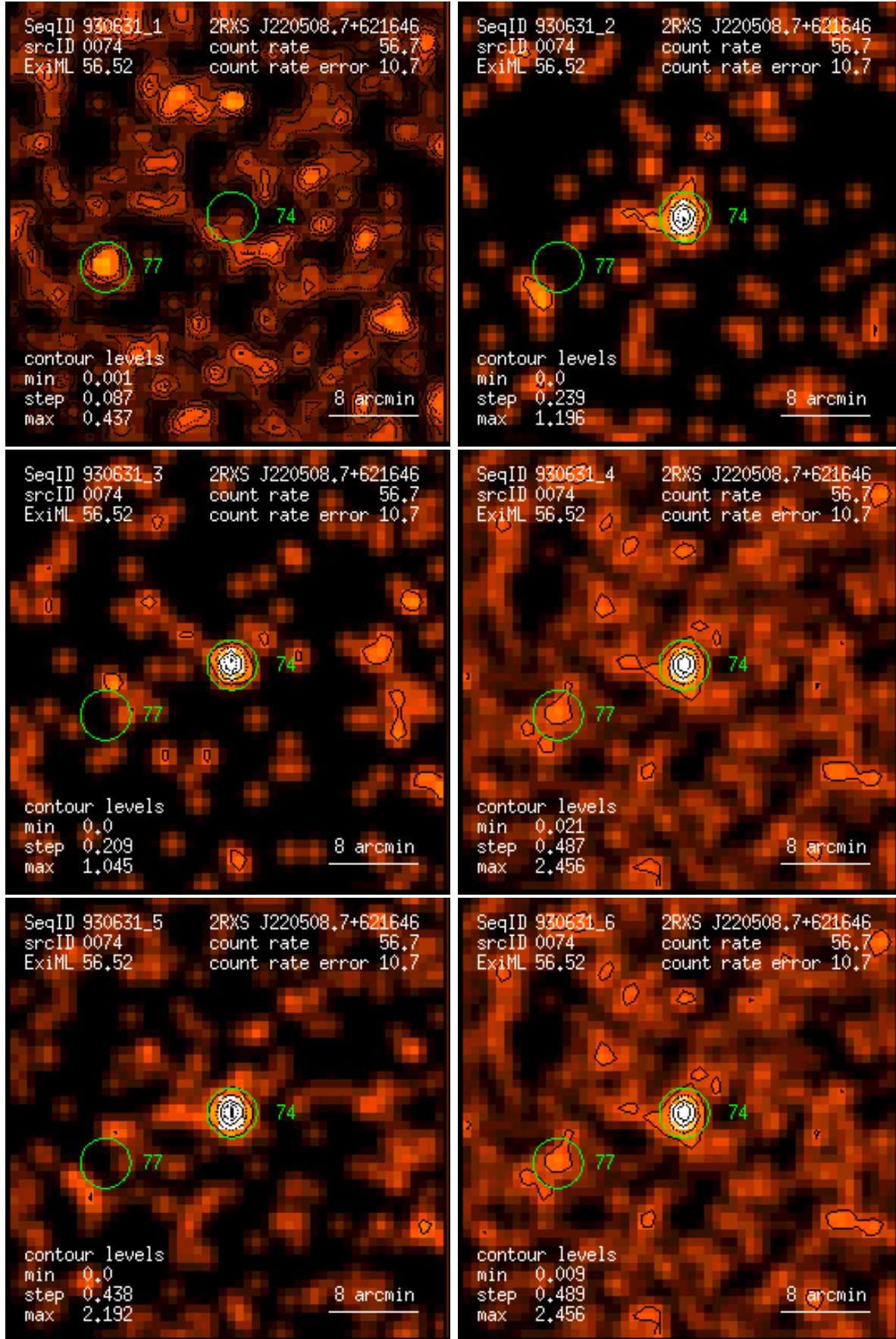
Figure 74: RASS 930631: detection 0074: band rate images, Gaussian filter: (1) PSPC channels 11 – 41, (2) 52 – 90, (3) 91 – 201, (4) 11 – 235, (5) 52 – 201, (6) 11 – 201. Broad band rates in counts/ks. Band rate contour levels in counts/ks/arcmin 2 .
