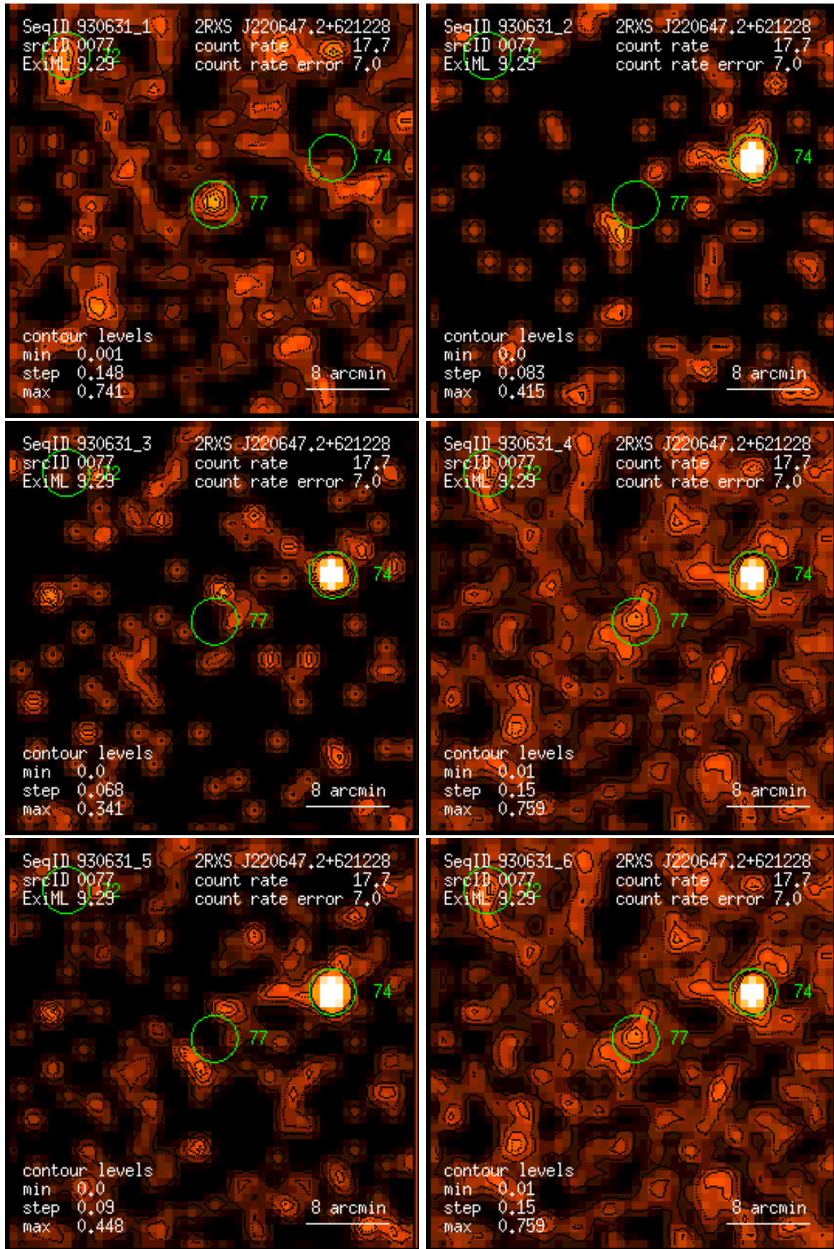
Figure 77: RASS 930631: detection 0077: band rate images, Gaussian filter: (1) PSPC channels 11 – 41, (2) 52 – 90, (3) 91 – 201, (4) 11 – 235, (5) 52 – 201, (6) 11 – 201. Broad band rates in counts/ks. Band rate contour levels in counts/ks/arcmin 2 .
