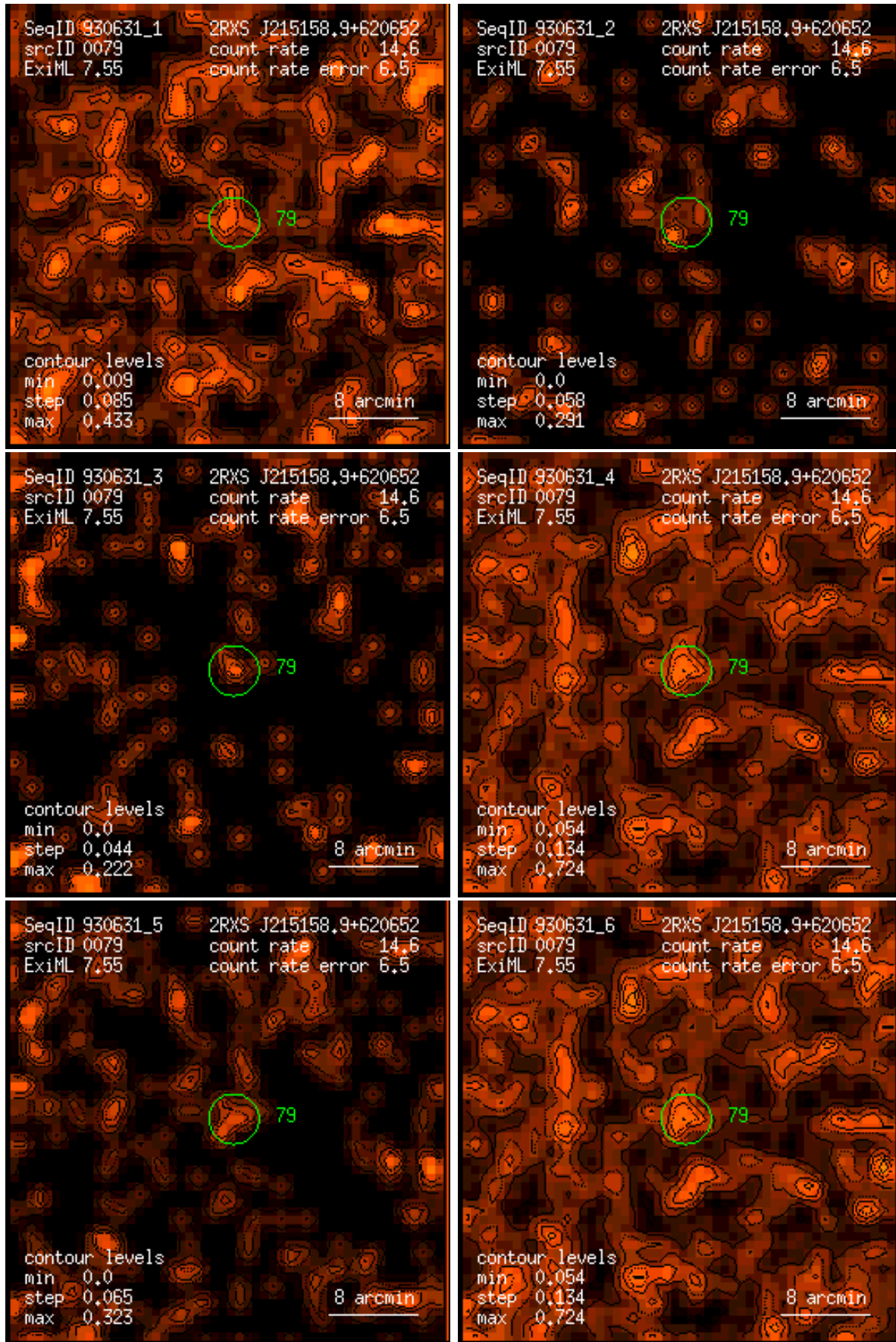
Figure 79: RASS 930631: detection 0079: band rate images, Gaussian filter: (1) PSPC channels 11 – 41, (2) 52 – 90, (3) 91 – 201, (4) 11 – 235, (5) 52 – 201, (6) 11 – 201. Broad band rates in counts/ks. Band rate contour levels in counts/ks/arcmin 2 .
