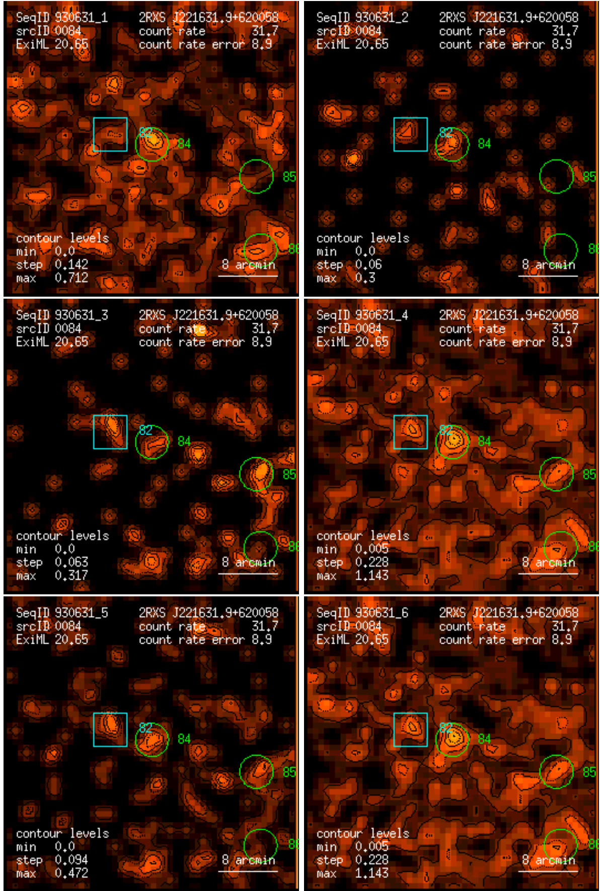
Figure 84: RASS 930631: detection 0084: band rate images, Gaussian filter: (1) PSPC channels 11 – 41, (2) 52 – 90, (3) 91 – 201, (4) 11 – 235, (5) 52 – 201, (6) 11 – 201. Broad band rates in counts/ks. Band rate contour levels in counts/ks/arcmin 2 .
