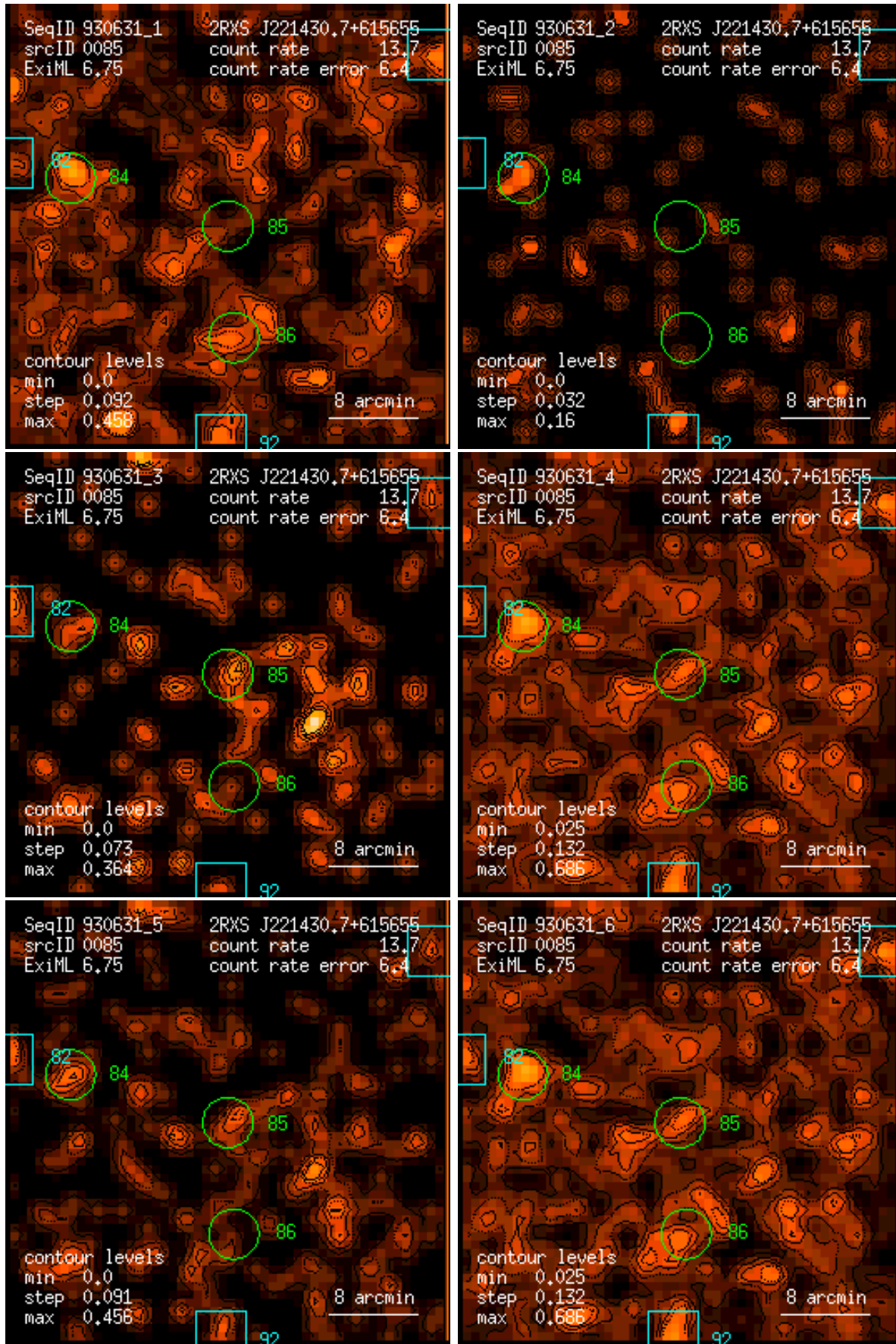
Figure 85: RASS 930631: detection 0085: band rate images, Gaussian filter: (1) PSPC channels 11 – 41, (2) 52 – 90, (3) 91 – 201, (4) 11 – 235, (5) 52 – 201, (6) 11 – 201. Broad band rates in counts/ks. Band rate contour levels in counts/ks/arcmin 2 .
