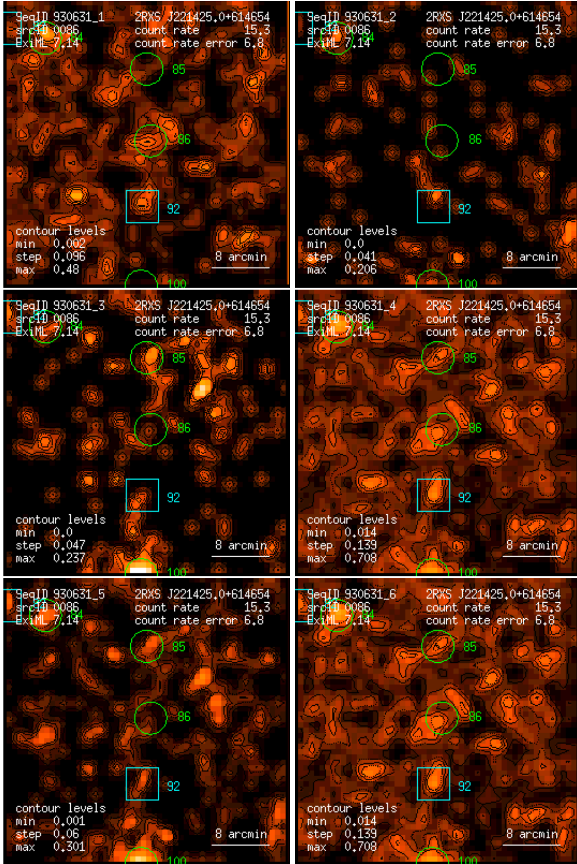
Figure 86: RASS 930631: detection 0086: band rate images, Gaussian filter: (1) PSPC channels 11 – 41, (2) 52 – 90, (3) 91 – 201, (4) 11 – 235, (5) 52 – 201, (6) 11 – 201. Broad band rates in counts/ks. Band rate contour levels in counts/ks/arcmin 2 .
