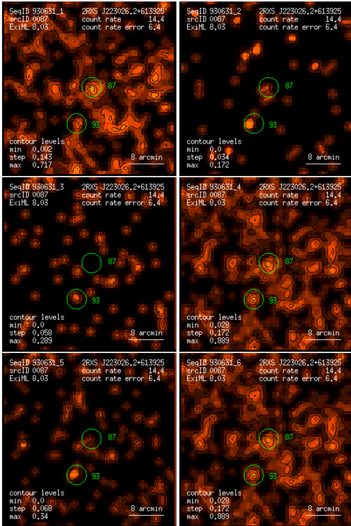
Figure 87: RASS 930631: detection 0087: band rate images, Gaussian filter: (1) PSPC channels 11 – 41, (2) 52 – 90, (3) 91 – 201, (4) 11 – 235, (5) 52 – 201, (6) 11 – 201. Broad band rates in counts/ks. Band rate contour levels in counts/ks/arcmin 2 .
