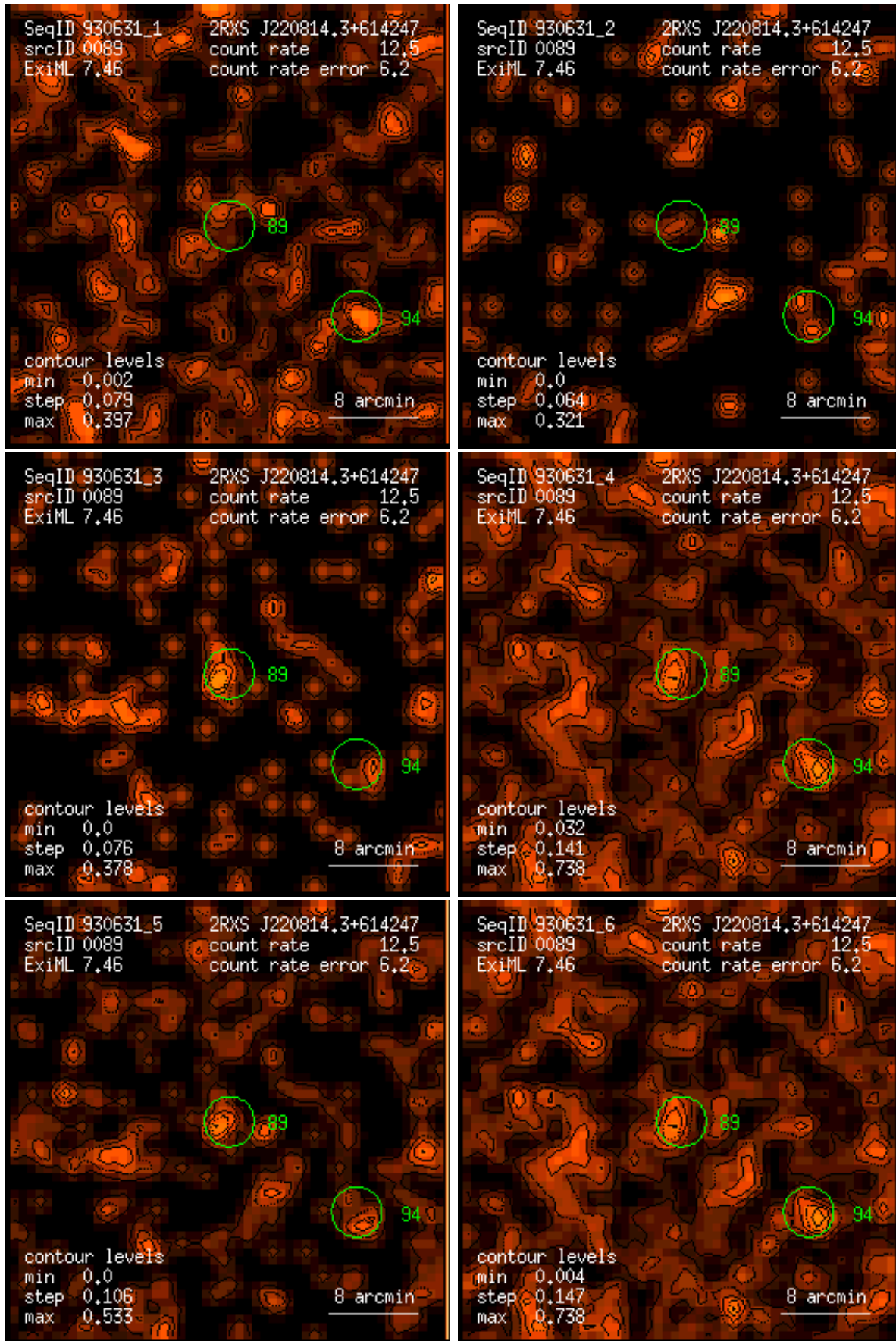
Figure 89: RASS 930631: detection 0089: band rate images, Gaussian filter: (1) PSPC channels 11 – 41, (2) 52 – 90, (3) 91 – 201, (4) 11 – 235, (5) 52 – 201, (6) 11 – 201. Broad band rates in counts/ks. Band rate contour levels in counts/ks/arcmin 2 .
