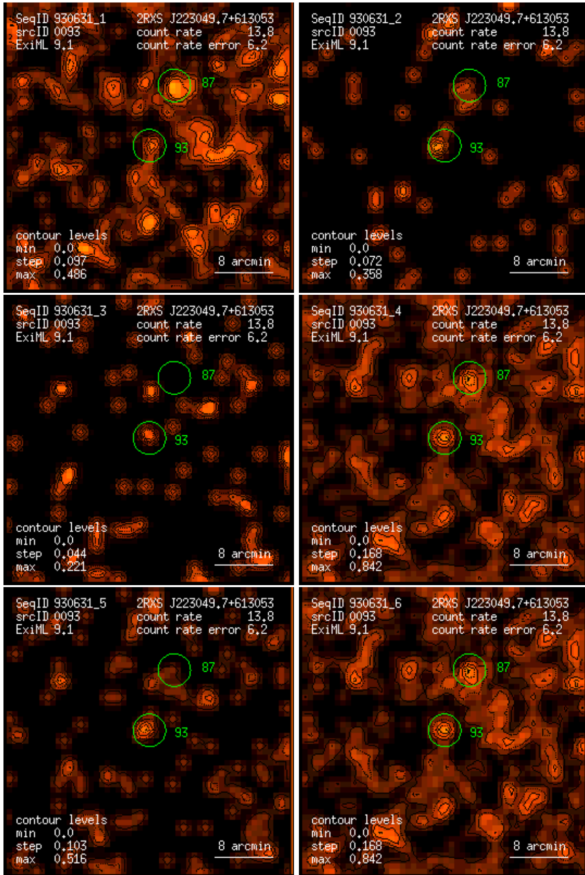
Figure 93: RASS 930631: detection 0093: band rate images, Gaussian filter: (1) PSPC channels 11 – 41, (2) 52 – 90, (3) 91 – 201, (4) 11 – 235, (5) 52 – 201, (6) 11 – 201. Broad band rates in counts/ks. Band rate contour levels in counts/ks/arcmin 2 .
