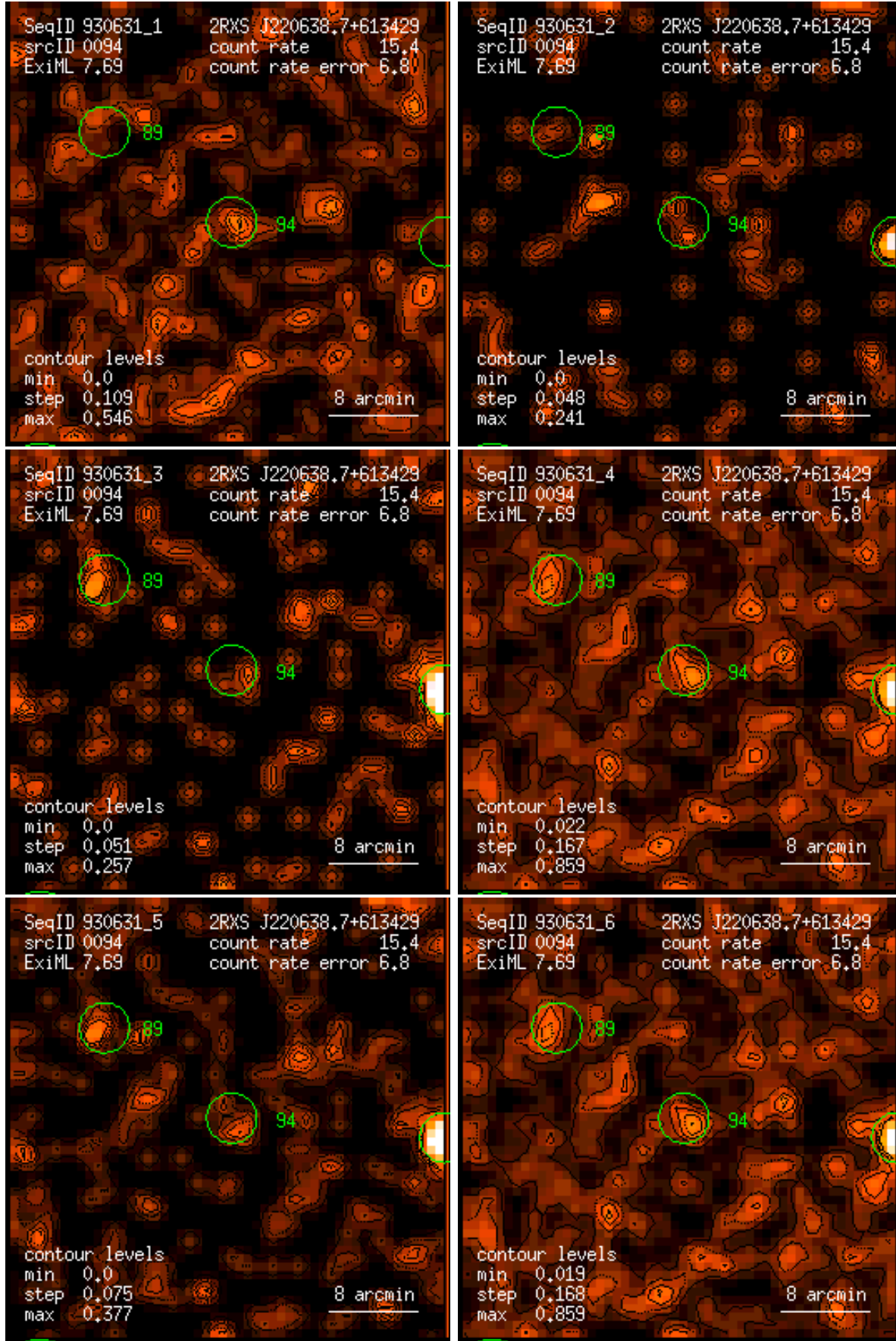
Figure 94: RASS 930631: detection 0094: band rate images, Gaussian filter: (1) PSPC channels 11 – 41, (2) 52 – 90, (3) 91 – 201, (4) 11 – 235, (5) 52 – 201, (6) 11 – 201. Broad band rates in counts/ks. Band rate contour levels in counts/ks/arcmin 2 .
