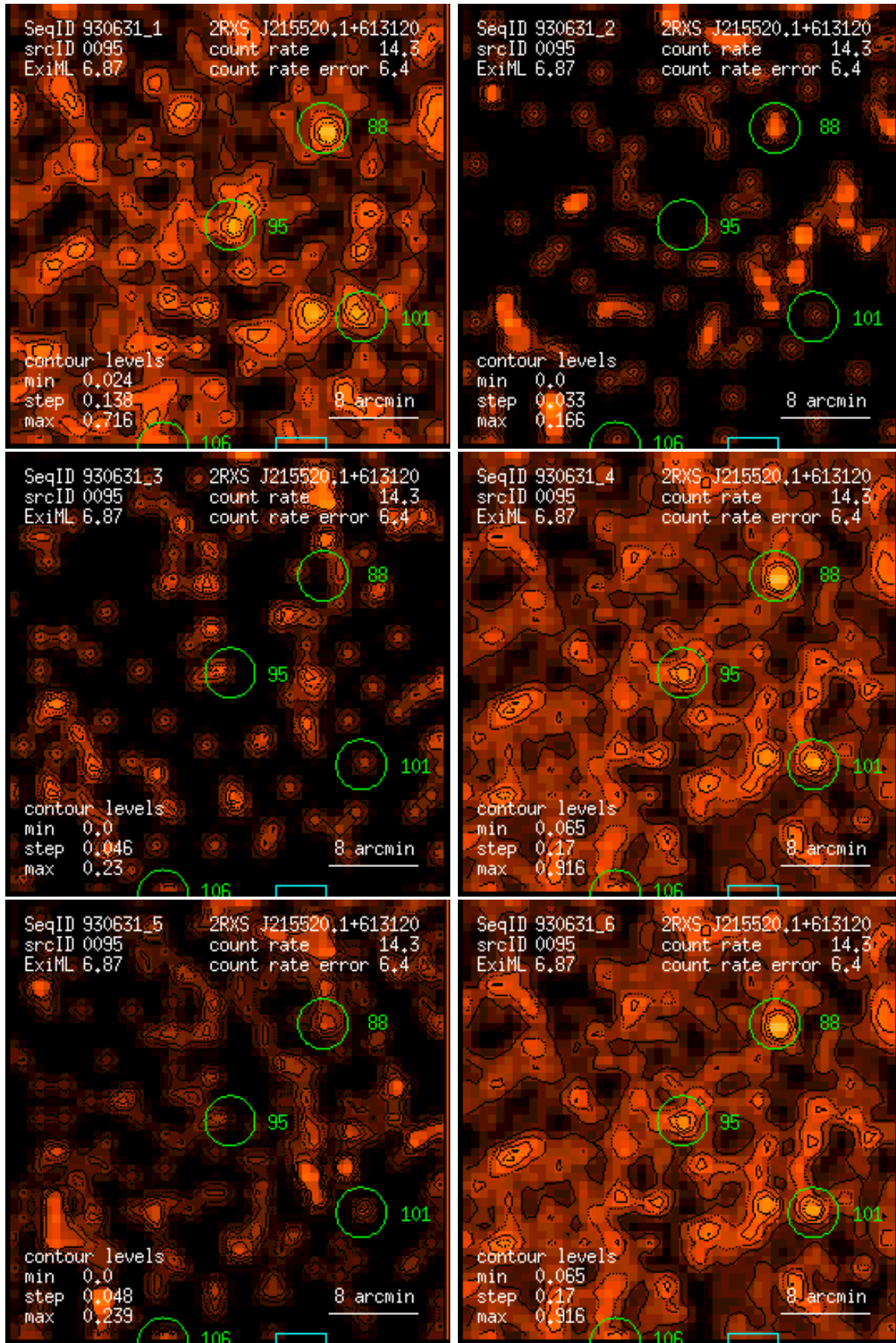
Figure 95: RASS 930631: detection 0095: band rate images, Gaussian filter: (1) PSPC channels 11 – 41, (2) 52 – 90, (3) 91 – 201, (4) 11 – 235, (5) 52 – 201, (6) 11 – 201. Broad band rates in counts/ks. Band rate contour levels in counts/ks/arcmin 2 .
