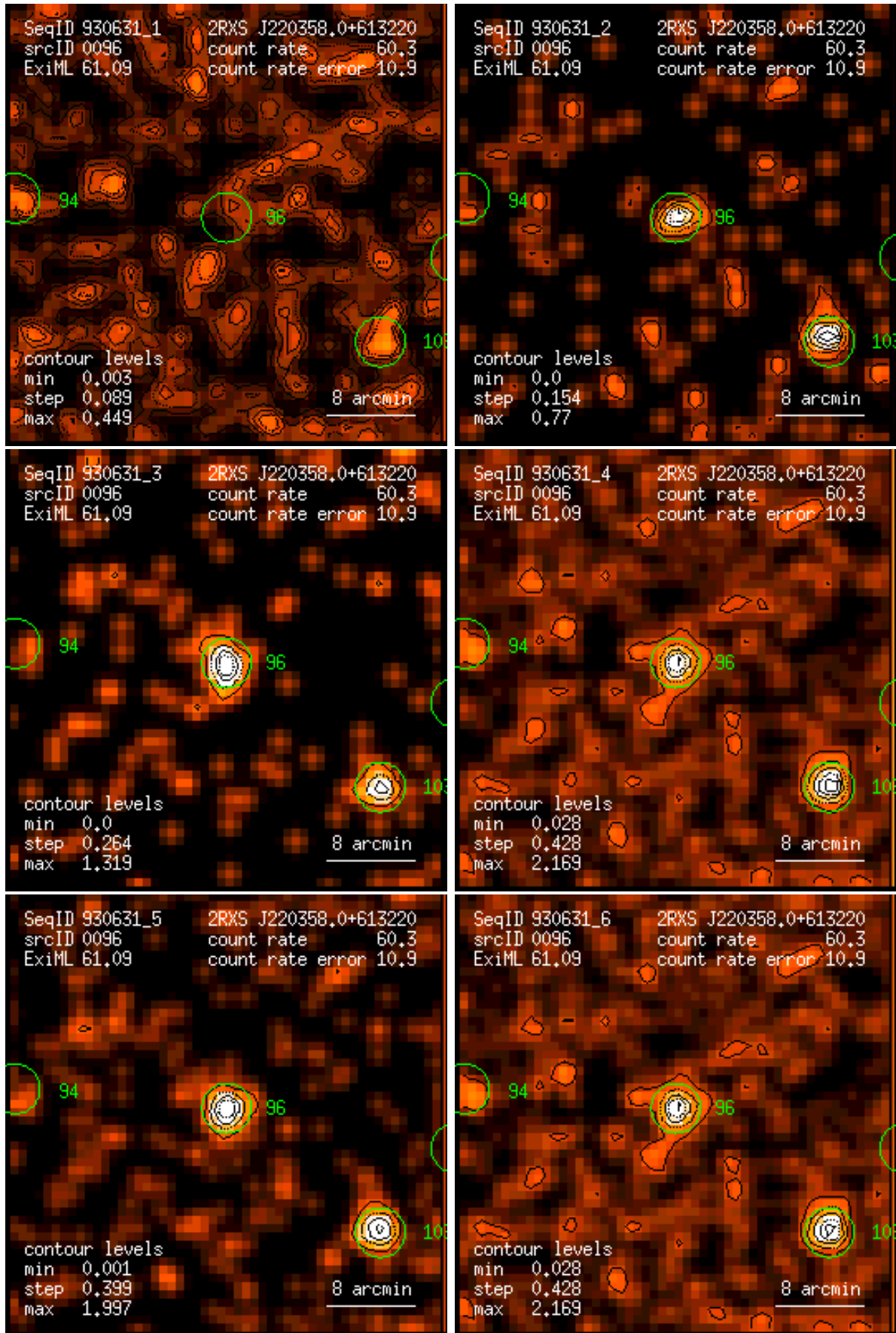
Figure 96: RASS 930631: detection 0096: band rate images, Gaussian filter: (1) PSPC channels 11 – 41, (2) 52 – 90, (3) 91 – 201, (4) 11 – 235, (5) 52 – 201, (6) 11 – 201. Broad band rates in counts/ks. Band rate contour levels in counts/ks/arcmin 2 .
